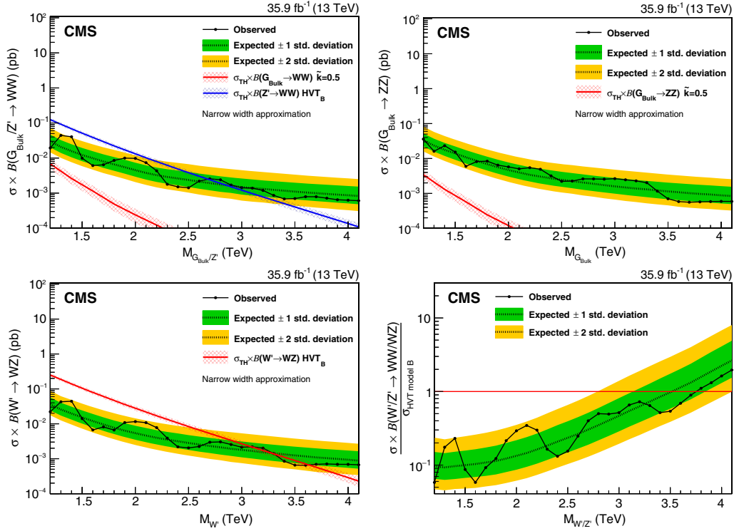
FIG. 6. Observed (black solid) and expected (black dashed) 95% C.L. upper limits on the production cross section of a narrow-width resonance decaying to a pair of vector bosons for different signal hypotheses. Limits are set (upper left plot) on a spin-1 neutral Z' and a spin-2 resonance decaying into WW , and compared with the prediction of the HVT model B (blue line) and a bulk graviton model with \tilde{k} = 0.5 (red line). Limits are also set in the context of a bulk graviton decaying into ZZ (upper right) with \tilde{k} = 0.5 and a spin-1 charged resonance decaying into WZ (lower left) and compared with the predictions of the models. Signal cross section uncertainties are displayed as cross-hatched bands. The plot on the lower right shows the 95% exclusion bounds on the signal strength for the triplet hypothesis of the HVT model B.
