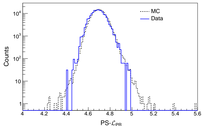
FIG. 2. Comparison of the distributions of the \text{PS-L}_{\text{PR}} parameter for ^{214}\text{Bi} events extracted from data (blue, continuous line) and generated using MC (black, dashed line). The MC sample of ^{214}\text{Bi} was generated using the same spatial distribution of the ^{214}\text{Bi} events of the data. The simulation also takes into account the proper values of the working channels N'(t) .
