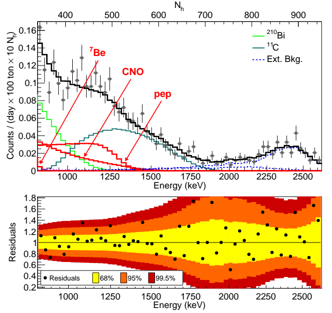
FIG. 10. TFC-subtracted energy spectrum zoomed between 800 keV and 2700 keV after applying stringent selection cuts on the radial distribution ( R < 2.4 m) and on the pulse-shape variable distribution ( PS-\mathcal{L}_{PR} < 4.8 ) to better see features due to pep vs interactions. The residuals (bottom plot) are the ratio between the data and the fit model.
