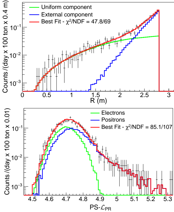
FIG. 8. An example of the multivariate fit showing the radial (top) and the PS-\mathcal{L}_{PR} (bottom) distributions of the events (black crosses) from the TFC-subtracted spectrum, in the energy intervals N_h > 290 and 409 < N_h < 645 , respectively.
