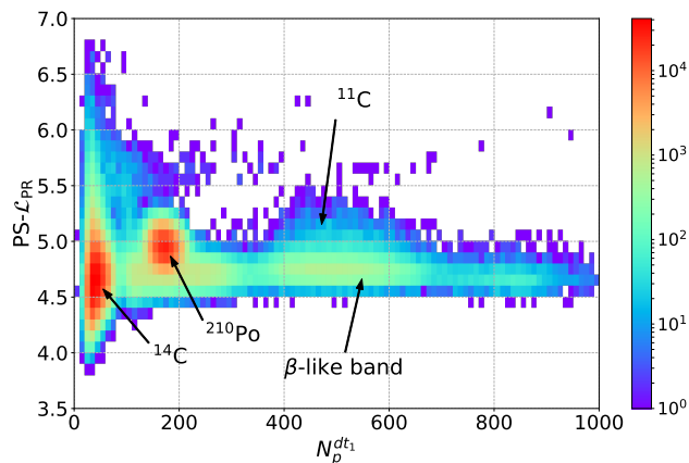
FIG. 4. Distribution of \text{PS-L}_{\text{PR}} pulse-shape discriminator as a function of N_p^{dt1} energy estimator. The plot is built using the entire set of data surviving the selection cuts described in Sec. II. The comparison with Fig. 3 allows to identify the range of values belonging to the \beta^- -like band indicated by the arrow.
