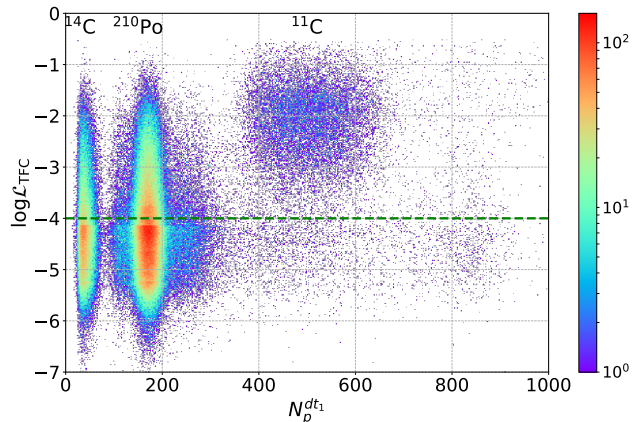
FIG. 1. Distribution of \log(\mathcal{L}_{\text{TFC}}) as a function of the N_p^{dt1} energy estimator. The plot is built using the entire set of data surviving the selection cuts described in Sec. II. The regions dominated by the abundant internal background of ^{14}\text{C} and ^{210}\text{Po} are indicated by the corresponding labels. The green-dashed horizontal line represents the \mathcal{L}_{\text{TFC}} -threshold, above/below which the events are assigned to the TFC-tagged/subtracted energy spectrum. It is clearly visible that the majority of the events of the ^{11}\text{C} energy decay spectrum lies above this threshold.
