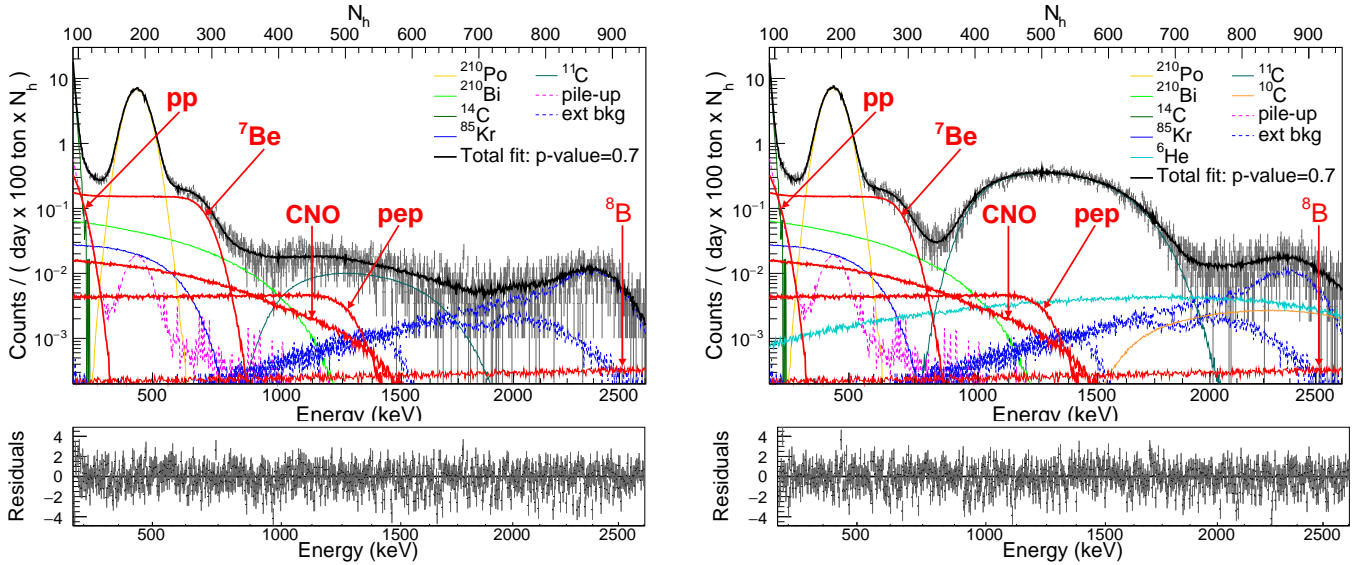
FIG. 7. Multivariate fit results (an example obtained with the MC method) for the TFC-subtracted (left) and the TFC-tagged (right) energy spectra, with residuals. The sum of the individual components from the fit (black lines) is superimposed on the data (grey points). The analysis has been performed using N_h as energy estimator and the transformation to keV-energy scale was performed only for the plotting purposes. The residuals are calculated in every bin as the difference between the data counts and the fit result, divided by the square root of the data counts.
