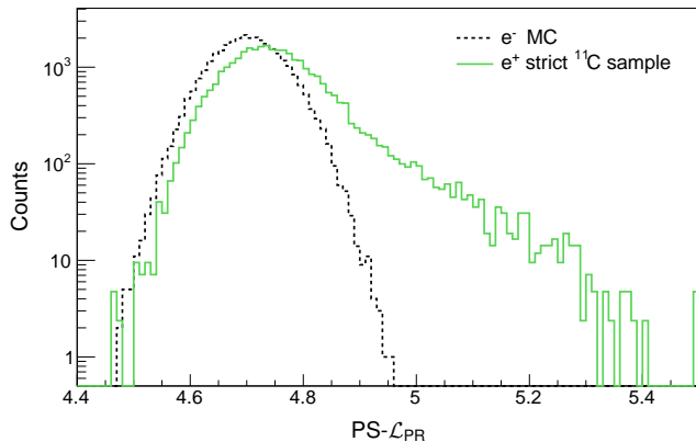
FIG. 3. Comparison of the distributions of the \text{PS-L}_{\text{PR}} variable for MC generated e^- events (black, dashed line) and for e^+ events selected from the data (green, continuous line). The latter events are a high-purity ^{11}\text{C} sample, obtained with the optimized TFC method, using very strict cuts on the energy and on the time correlation with the neutron and muon tracks.
