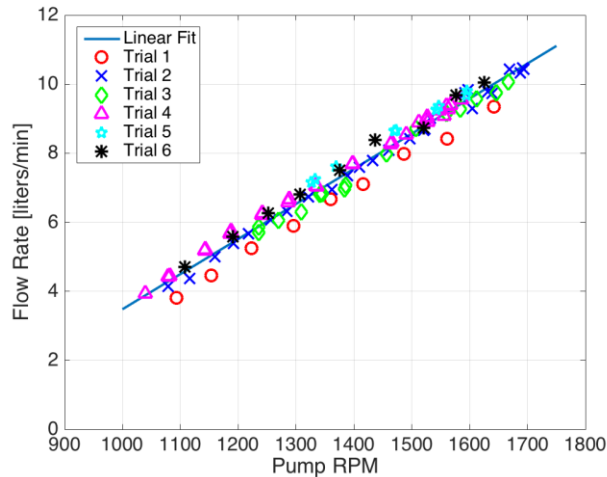
Figure 8 - The measured output of the LMX pump with B = 0 [T]. The pump provided repeatable flow rates over multiple days of testing.
