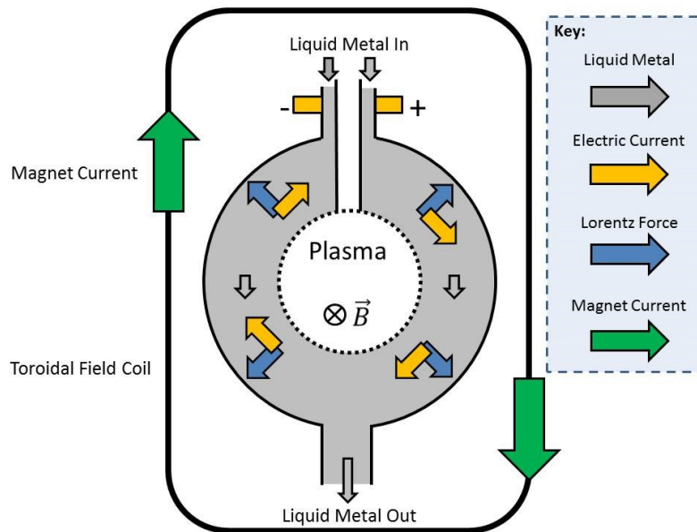
Figure 1 - A simple depiction of electromagnetically restrained liquid-metal within a tokamak. (Adapted from [11, 13].)
