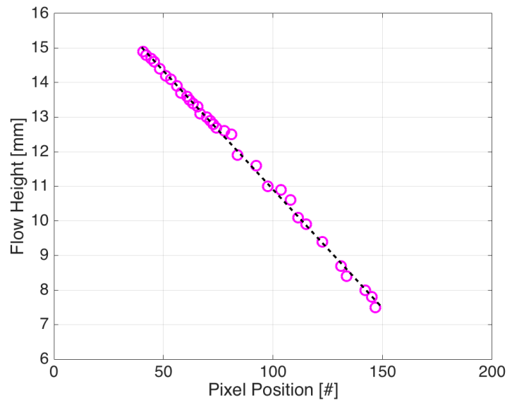
Figure 11 - Laser-sheet height calibration data. The points below a height of 12.5 [mm] correspond to galinstan levels that did not spill over the weir. When the depth of the galinstan was greater than 15 [mm] the laser-sheet data was calibrated using the extrapolated linear fit of the data. As detailed in Figure 2, the actual height change and the change on the laser-sheet videos scale using a constant coefficient.
