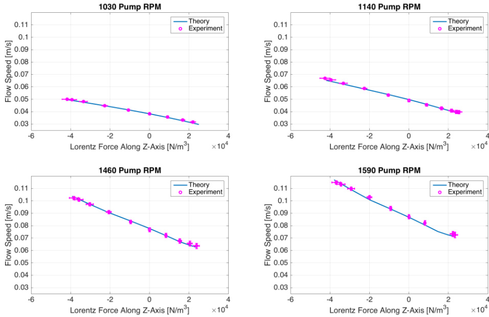
Figure 7 - Average flow velocity of liquid-metal as a function of applied Lorentz force. For this study, g = 9.80665 \text{ [m/s}^2\text{]} , \rho = 6400 \text{ [kg/m}^3\text{]} , w = 0.109 \text{ [m]} .
