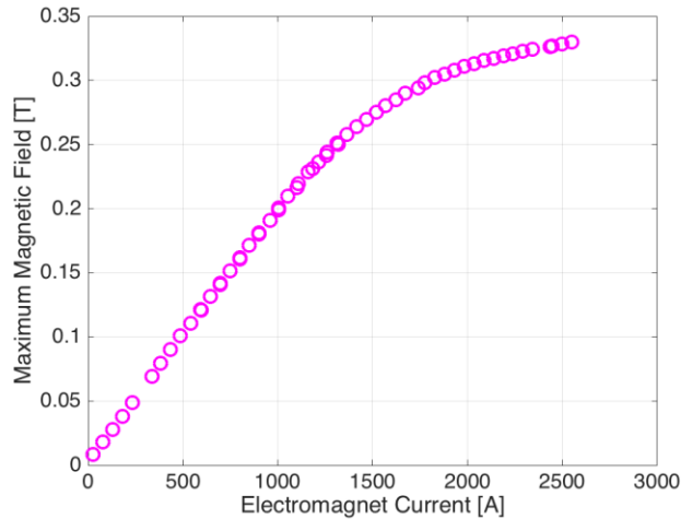
Figure 12 - The measured peak output of the electromagnet used in LMX. The cooling system on the magnet did not allow for steady-state operation using larger electromagnet currents.
