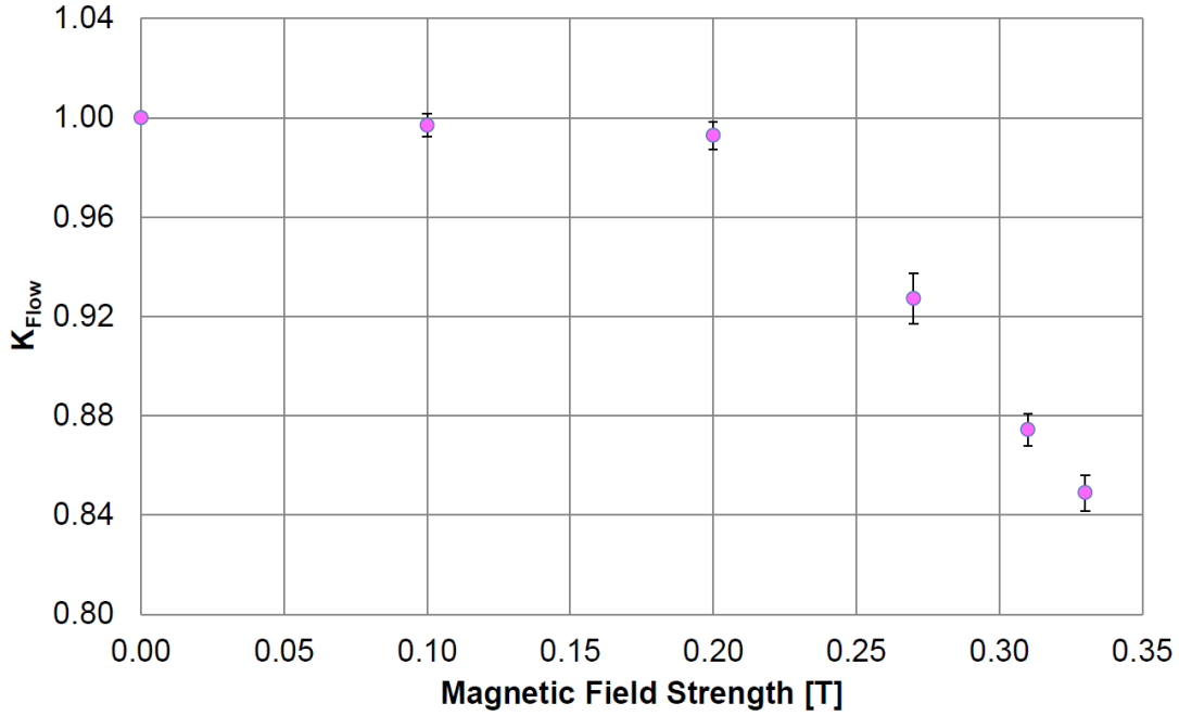
Figure 10 - The experimentally determined flow correction factor ( K_{Flow} ) that accounts for changes in pump performance resulting from MHD drag.
