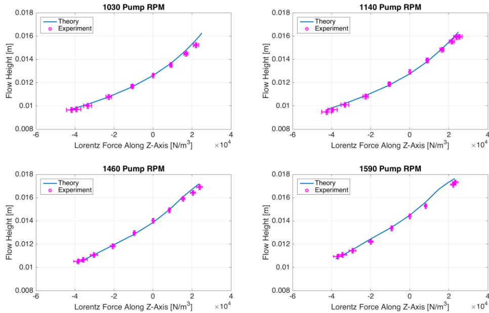
Figure 6 – Flow heights of liquid-metal as a function of applied Lorentz force. For this study, g = 9.80665 \text{ [m/s}^2\text{]} , \rho = 6400 \text{ [kg/m}^3\text{]} , w = 0.109 \text{ [m]} . (Note: Y-axis error bars correspond to a constant, maximum expected error of \pm 200 \text{ [}\mu\text{m]} .)
