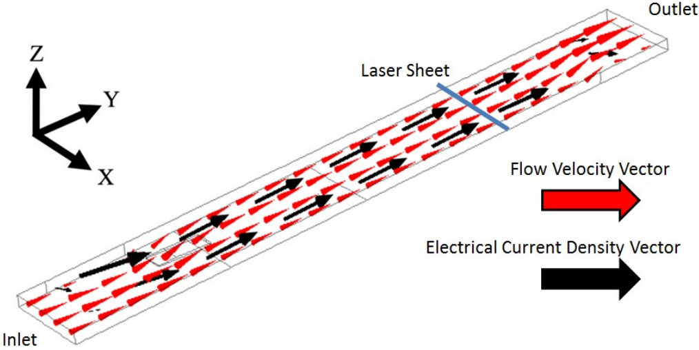
Figure 4 - A COMSOL simulation showing the electrical current density vector and the liquid metal flow velocity vector. Both profiles are uniform towards the center of the duct where the height measurements were taken (Pump RPM = 1600, B = 0.3 [T], I = 70 [A]).
