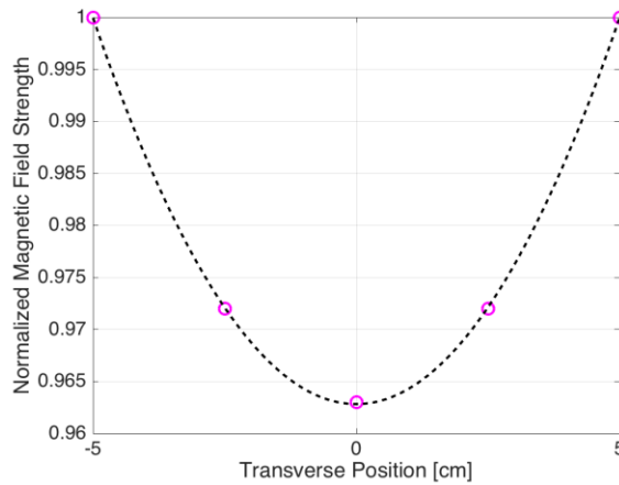
Figure 13 - The normalized magnetic field strength across the acrylic channel used in LMX. These data can be represented using a parabolic fit.
