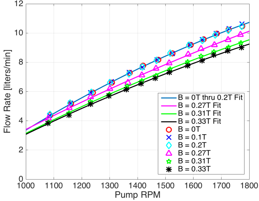
Figure 9 – The measured LMX pump performance with magnetic field ranging from 0-0.33 [T].
