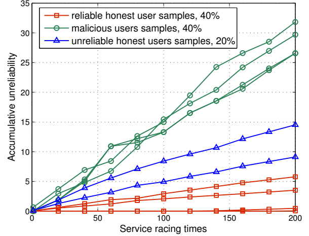
Fig. 4. The accumulative unreliability of user samples of three types.
