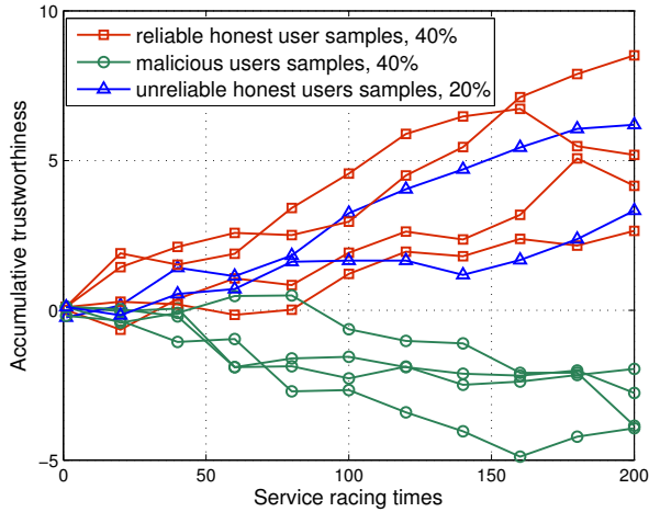
(b) Binary quadratic scoring
