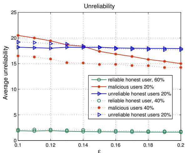
Fig. 6. The average unreliability of different types of users versus the percentage of each user type and \epsilon .
