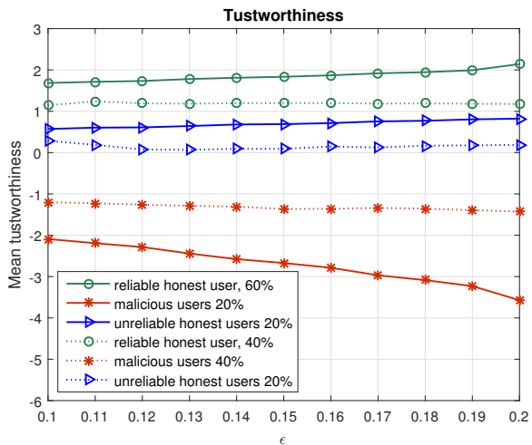
(a) Binary logarithmic scoring
