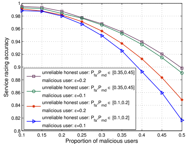
Fig. 7. The service rating accuracy versus the the percentage of each user type, error rates of judgement P_{fa} , P_{md} and \epsilon .
