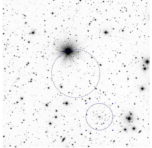
Fig. 11. PSZ1 G066.01-23.30 RTT150 i' -band image centred on the Planck SZ source coordinates, dashed 2' radius circle shows approximate Planck SZ source coordinates uncertainty. The position of the optical galaxy cluster is shown with a solid circle.
