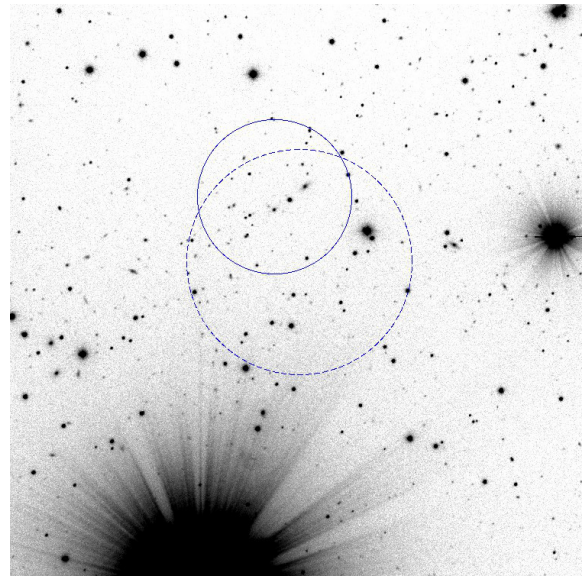
Fig. 16. PSZ1 G103.50+31.36 RTT150 r' -band image, dashed circle ( 2' radius) shows the location of Planck SZ source. The SZ source may be identified with the galaxy group shown in the solid circle. However, there is also a very bright star ( m_V = 5.8 ) at the edge of the field, 5/6 from the Planck position and detected by Planck , which most probably affects the SZ signal.
