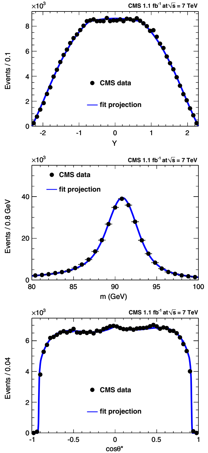
FIG. 10 (color online). Distributions of Y (top), m (middle), and \cos\theta^* (bottom) in the analysis of q\bar{q} \rightarrow \gamma^*/Z \rightarrow \mu^-\mu^+ events from CMS (points). The lines show the projections of the probability density functions.
