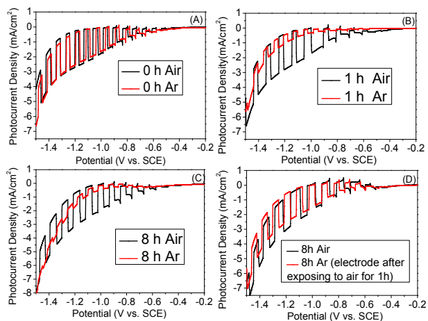
Figure 6. Linear sweep voltammetry of CuRhO 2 electrodes: (A) Before electrolysis under chopped light conditions. (B) After electrolysis for 1 h. (C) After electrolysis for 8 h. (D) The electrode, after electrolysis for 8 h was exposed to air for 1 h at 100 °C.
