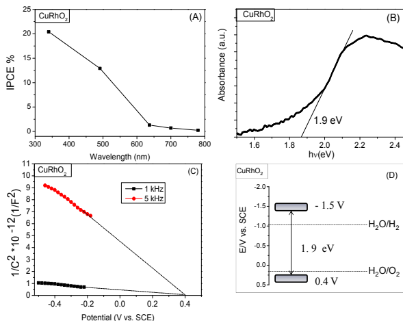
Figure 2. (A) IPCE plots obtained at -0.9 V vs. SCE under the air-saturated condition. (B) UV-Vis-NIR absorption spectrum of \text{CuRhO}_2 . (C) Mott-Schottky plots at 1 kHz and 5 kHz measured under dark conditions. (D) The CB and VB positions of \text{CuRhO}_2 compared with the water redox potentials at \text{pH}=14 .
