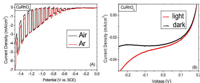
Figure 1. (A) Linear Sweep Voltammetry with a freshly made CuRhO 2 electrode measured under chopped light in 1 M NaOH purged with Ar (red) and Air (black) (scan rate, 100 mV/s) (B)
