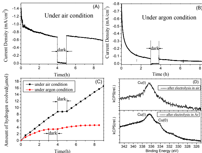
Figure 4. (A) Photoelectrolysis: cathodic current density vs. time in an air-saturated solution. (B) Photoelectrolysis: cathodic photocurrent density vs. time in an argon-saturated solution. (C) \text{H}_2 evolution using \text{CuRhO}_2 as a photocathode with an applied potential of -0.90 V in argon- or air-saturated 1 M NaOH solutions under visible light irradiation. (D) XPS characterization of \text{CuRhO}_2 electrodes surface after electrolysis under air and argon.
