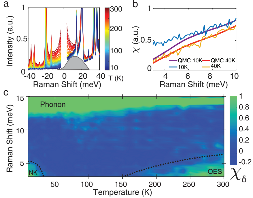
Figure 1: Effects of non-Kitaev Terms (a) Temperature dependent Raman intensity of \alpha - \text{RuCl}_3 in XY polarization. Both Stokes and anti-Stokes data are collected from 10 K to 300 K with 5 K steps below 120 K and 10 K steps above. the gray shade is indicates the magnetic continuum excitation. (b) The measured Raman susceptibility in XY polarization of \alpha - \text{RuCl}_3 at 10 K (blue line) compared with the calculated result of the pure Kitaev limit (purple line) at the same temperature. The enhanced signal at low energies results from the non-Kitaev interactions in the system. By 40 K there is nearly perfect agreement between the Raman data (yellow line) and the QMC calculation (red line), indicating the non-Kitaev terms are not relevant in this energy and temperature range. (c) The temperature and energy dependent map of \chi_\delta ( \chi_\delta = \chi_{\text{measured}} - \chi_{\text{QMC}} ). \chi_\delta at low temperature and low energy range shows the temperature and energy boundary of non-Kitaev (NK) interactions in the system. \chi_\delta at the high temperature and low energy range indicates the quasi-elastic scattering (QES) in the system.
