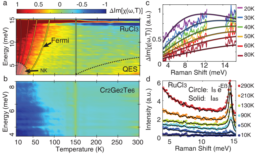
Figure 2: The normalized Raman susceptibility and detailed balance (a) Raman susceptibility of RuCl 3 , \Delta \text{Im}[\chi(\omega, T)] = \text{Im}[\chi(\omega, T)] - \text{Im}[\chi(\omega, 150 \text{ K})] . The curves with black outlines are the contour plots of the Fermi function ( \Delta n_F(\omega/2, T) = n_F(\omega/2, 150) - n_F(\omega/2, T) ). Both data and the prediction are normalized to their maximum values. The agreement between the two confirms that Raman creates magnetic excitations that are made of pairs of fermions. The upturn of the Raman intensity in the high temperature and low energy range results from thermal fluctuations of the magnetism (quasi-elastic scattering). (b) Raman susceptibility of a similar magnet, Cr 2 Ge 2 Te 6 , where, opposite to \alpha -RuCl 3 , \Delta \text{Im}[\chi(\omega, T)] is negative and does not match n_F(\omega/2, T) . (c) Comparison of n_F(\omega/2, T) and \Delta \text{Im}[\chi(\omega, T)] of RuCl 3 at fixed temperatures. The agreement further confirms the excitations are fermionic. (d) The excellent agreement between Stokes and anti-Stokes spectra of \alpha -RuCl 3 when normalized by the Boltzmann factor demonstrates the absence of laser heating.
