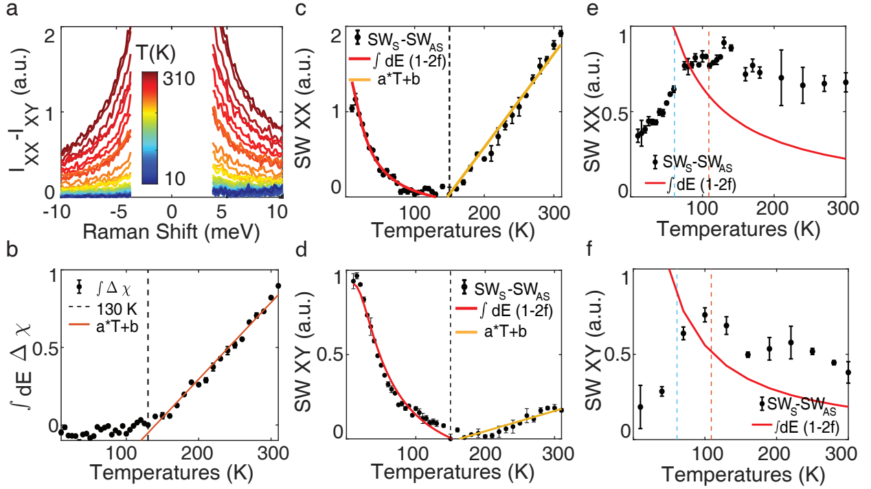
Figure 3: Limit of Fermi statistics (a) The continuum in \alpha -RuCl 3 due to fractional particles is removed by taking the difference between XY and XX intensities. This confirms the continuum is consistent with predictions of the Kitaev model, and the high temperature response is from quasi-elastic scattering (i.e. Lorentzian times a Bose factor). (b) The integration of the Raman susceptibility(3meV - 8meV) with only the quasi-elastic scattering response, reveals a linear T behavior above 150 K and temperature independent behavior below. (c & d) Integrated spectral weight(3meV - 8meV) of \text{Im}[\chi(\omega, T)] , reveals Fermi statistics in \alpha -RuCl 3 below \approx 100 K (solid red line) in XX and XY polarizations. Above 150 K the response is linear in temperature due to the quasi-elastic scattering (yellow lines). The spectral weight(3meV - 8meV) from Cr 2 Ge 2 Te 6 (e & f) is enhanced up to T_C (blue dashed line) but the temperature dependence above does not fit that expected for fermions (solid red line).
