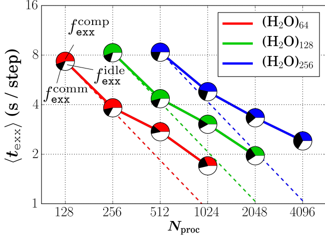
FIG. 8. Strong-scaling analysis of the MPI internode parallelization level in exx during CPMD simulations of liquid water at the hybrid PBE0 level on the Mira IBM Blue Gene/Q platform. For a fixed system size ( i.e. , (H_2O)_{64} (red line), (H_2O)_{128} (green line), and (H_2O)_{256} (blue line)), the walltime spent in the exx module ( \langle t_{\text{exx}} \rangle in s/step, averaged over 50 CPMD steps) is plotted versus the number of MPI processes ( N_{\text{proc}} ), which were varied to include \zeta = N_{\text{proc}}/N_o = 1/2, 1, 2, 4 . For reference, ideal strong-scaling timings were plotted as dashed lines for each system size, and were computed with respect to the corresponding \zeta_{\text{ref}} = 1/2 timings. Pie plots were used to illustrate the fraction of \langle t_{\text{exx}} \rangle dedicated to computation events ( f_{\text{exx}}^{\text{comp}} , colored), communication overhead ( f_{\text{exx}}^{\text{comm}} , black), and processor idling ( f_{\text{exx}}^{\text{idle}} , white).
