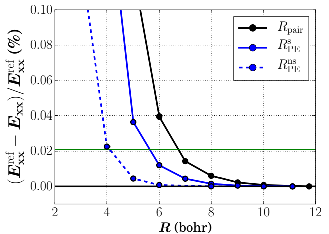
FIG. 6. Convergence of E_{xx} as a function of R_{\text{pair}} , R_{\text{PE}}^s , and R_{\text{PE}}^{\text{ns}} on a snapshot of liquid water containing (\text{H}_2\text{O})_{64} in a cubic cell with L = 23.52 Bohr. Relative errors (in %) with respect to E_{xx}^{\text{ref}} are evaluated individually by varying R_{\text{pair}} (solid black line), R_{\text{PE}}^s (solid blue line), and R_{\text{PE}}^{\text{ns}} (dashed blue line), while keeping all other parameters set to their maximum allowed values (see text for more details). An overall relative error of \approx 0.02\% corresponds to the default parameter values in QE ( i.e. , R_{\text{pair}} = 8.0 Bohr, R_{\text{PE}}^s = 6.0 Bohr, R_{\text{PE}}^{\text{ns}} = 5.0 Bohr), and is depicted by the solid green line.
