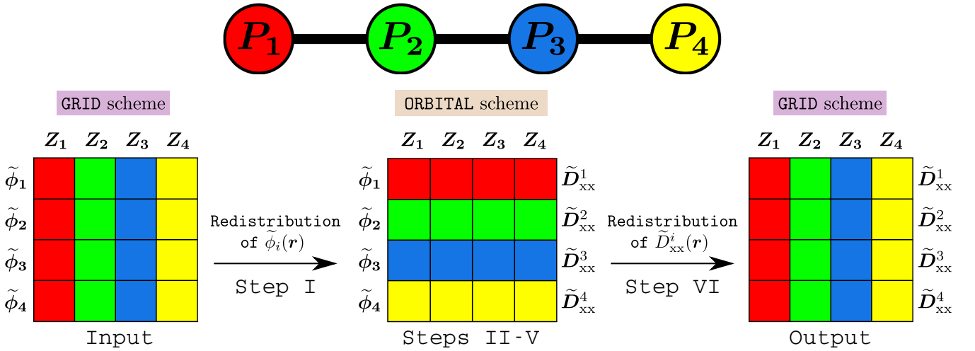
FIG. 3. Schematic illustration of the GRID and ORBITAL data distribution schemes in QE. For simplicity, we consider a system consisting of a single water molecule with N_o = 4 MLWFs ( \tilde{\phi}_i(\mathbf{r}) ), a simulation cell consisting of a real-space simple-cubic grid that has been partitioned into N_{\text{slab}} = 4 slabs along the z -direction ( Z_i ), and a pool of N_{\text{proc}} = 4 MPI processes ( P_i ). As depicted at the top of the figure, each of these MPI processes (and the corresponding data it holds in local memory) is assigned a color: P_1 (red), P_2 (green), P_3 (blue), and P_4 (yellow). As input into the exx module, the \tilde{\phi}_i(\mathbf{r}) are provided in the GRID scheme, in which a given MPI process, P_i , holds the data corresponding to all N_o MLWFs on one slab, Z_i , of the real-space grid. During Step I of the exx module (Sec. III C 1), the \tilde{\phi}_i(\mathbf{r}) are redistributed according to the ORBITAL scheme, in which a given MPI process, P_i , holds the data corresponding to only one MLWF, \tilde{\phi}_i(\mathbf{r}) , across all N_{\text{slab}} slabs of the real-space grid. As described in Secs. III C 2–III C 5, Steps II–V involve selective communication of the \tilde{\phi}_i(\mathbf{r}) between MPI processes and computation of all EXX-related quantities ( E_{\text{xx}} and \{\tilde{D}_{\text{xx}}^i(\mathbf{r})\} ). At the end of Step V, the \{\tilde{D}_{\text{xx}}^i(\mathbf{r})\} are stored according to the ORBITAL scheme, and are redistributed back to the GRID scheme during Step VI (Sec. III C 6), the final step of the exx module.
