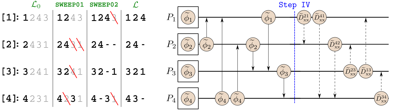
FIG. 4. Graphical depiction of the unique MLWF-pair list construction process and corresponding MLWF communication scheme in the exx module. For simplicity, we will again consider a single water molecule with N_o = 4 MLWFs ( \tilde{\phi}_i ) and a pool of N_{\text{proc}} = 4 MPI processes ( P_i ), i.e. , \zeta = 1 . Starting with the non-unique MLWF-pair list, \mathcal{L}_0 , which contains all possible permutations of overlapping MLWF pairs, the step-by-step procedure employed to transform \mathcal{L}_0 into the unique MLWF-pair list, \mathcal{L} , is depicted in the left panel. Since all of the MLWFs are mutually overlapping in a single water molecule, \mathcal{L}_0[i] contains \{j\} , the indices corresponding to all MLWFs (including j = i ), which have been sorted according to |\tilde{C}_i - \tilde{C}_j| . During the process of reducing \mathcal{L}_0 to \mathcal{L} , i is always selected (bold black font) to remain in \mathcal{L}_0[i] , while the remaining non-unique indices are shown in gray. In the first sweep (SWEEP01) of Algorithm 1, the next element j \in \mathcal{L}_0[i] is selected to remain in \mathcal{L}_0[i] , while the now redundant index i is removed (red slash) from \mathcal{L}_0[j] . During the first sweep in this example, the indices 2, 4, 2, 3 were selected to remain in \mathcal{L}_0[1], \mathcal{L}_0[2], \mathcal{L}_0[3], \mathcal{L}_0[4] , while the corresponding redundant indices, 1, 2, 3, 4, were removed from \mathcal{L}_0[2], \mathcal{L}_0[4], \mathcal{L}_0[2], \mathcal{L}_0[3] . This process is repeated until all of the MLWF-pair redundancy is removed from \mathcal{L}_0 , upon which one is left with the final \mathcal{L} . For a single water molecule, only two sweeps are required to reach this stage; at that point, all of the unique MLWF pairs have been assigned to a given \mathcal{L}[i] , and no redundant indices remain. With each MLWF stored according to the ORBITAL data distribution scheme (in which \tilde{\phi}_i is assigned to P_i ), the final \mathcal{L} determines how the computational workload will be distributed among the pool of available MPI processes. Even in this simple example, there exists a mismatch in the number of pairs assigned to each process, with three MLWF pairs assigned to P_1 and P_3 , and only two MLWF pairs assigned to P_2 and P_4 . Such discrepancies are expected (even for the most homogeneous systems) and lead to an imbalance in the computational workload. By virtue of the ORBITAL data distribution scheme, \mathcal{L} also determines the corresponding MLWF communication protocol, which is depicted in the right panel for the single water molecule. After a given \tilde{\phi}_j is directly communicated to P_i , this MPI process forms \tilde{\rho}_{ij} , solves the corresponding PE for \tilde{v}_{ij} (depicted by the blue dashed line), and computes the \langle ij \rangle -pair contribution to E_{\text{xx}} , \tilde{D}_{\text{xx}}^{ij} , and \tilde{D}_{\text{xx}}^{ji} (which is sent back to P_j ). As an example, consider \mathcal{L}[2] , which contains two indices (2, 4). Since P_2 already holds \tilde{\phi}_2 , \tilde{\rho}_{22} (required for computing \tilde{v}_{22} ) can be constructed locally without the need for any interprocess communication. To construct \tilde{\rho}_{24} (and hence \tilde{v}_{24} ), \tilde{\phi}_4 is sent from P_4 to P_2 (solid arrow). After the corresponding \tilde{D}_{\text{xx}}^{42} is formed, it is shipped back to P_4 (dashed arrow). Besides this straightforward dependency between receiving an MLWF and computing the corresponding EXX contributions to the wavefunction forces, the communication in the exx module has no discernible time axis in the figure above.
