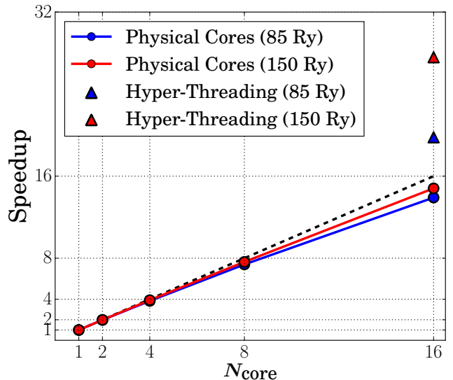
FIG. 10. Strong-scaling analysis of the OpenMP intranode parallelization level in exx during CPMD simulations of (\text{H}_2\text{O})_{64} at the hybrid PBE0 level on the Mira IBM Blue Gene/Q platform. For a fixed system and basis set size ( i.e. , (\text{H}_2\text{O})_{64} with a planewave kinetic energy cutoff of 85 Ry (blue line) and 150 Ry (red line)), the speedup in the walltime spent in Step IV: Solution of Poisson’s Equation of Fig. 2 ( \langle t_{\text{exx}}^{\text{Step IV}} \rangle , averaged over 50 CPMD steps) is plotted versus the number of physical cores, which were varied to include N_{\text{thread}} = N_{\text{core}} = 1, 2, 4, 8, 16 . Beyond the maximum number of physical cores ( N_{\text{core}} = 16 ) per node on Mira , the OpenMP intranode parallelization level can further utilize hyperthreading technology to access up to N_{\text{thread}} = 64 (hyper)threads (depicted by the blue and red triangles). For reference, the ideal strong-scaling performance (using up to N_{\text{core}} = 16 ) was plotted as a dashed line, and normalized to unity for N_{\text{core}} = 1 .
