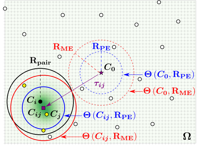
FIG. 5. Graphical depiction of the proto-subdomains used in the exx module. Dots are used to denote the MLWF centers, \tilde{\mathbf{C}}_i , which are approximated by the closest points, \mathbf{C}_i , on the real-space grid, \Omega . The dashed blue and red circles bound the two concentric spherical proto-subdomains, \Theta(\mathbf{C}_0, R_{\text{PE}}) and \Theta(\mathbf{C}_0, R_{\text{ME}}) , which are assembled around \mathbf{C}_0 (purple star) with radii R_{\text{PE}} and R_{\text{ME}} , respectively. Pair-exchange interactions involving \tilde{\phi}_i(\mathbf{r}) include all overlapping MLWFs (yellow dots), whose centers are located within a distance, R_{\text{pair}} , of \tilde{\mathbf{C}}_i \approx \mathbf{C}_i (black dot) that is large enough to account for all \tilde{\phi}_k(\mathbf{r}) with \Omega_{ik} \neq \emptyset . For the overlapping \langle ij \rangle pair, the \Theta(\mathbf{C}_0, R_{\text{PE}}) and \Theta(\mathbf{C}_0, R_{\text{ME}}) proto-subdomains are translated across \Omega via a rigid grid offset, \tau_{ij} , to form \Theta(\mathbf{C}_{ij}, R_{\text{PE}}) and \Theta(\mathbf{C}_{ij}, R_{\text{ME}}) , which are centered at \tilde{\mathbf{C}}_{ij} \approx \mathbf{C}_{ij} (purple square). To evaluate the \langle ij \rangle contribution to all EXX-related quantities, the corresponding PE, \nabla^2 \tilde{v}_{ij}(\mathbf{r}) = -4\pi \tilde{\rho}_{ij}(\mathbf{r}) , is solved for \tilde{v}_{ij}(\mathbf{r}) on the \Theta(\mathbf{C}_{ij}, R_{\text{PE}}) subdomain, which encompasses \Omega_{ij} , the support of \tilde{\rho}_{ij}(\mathbf{r}) (shaded in dark green). Boundary conditions for the PE (as well as the far-field \tilde{v}_{ij}(\mathbf{r}) ) are computed via a ME of \tilde{\rho}_{ij}(\mathbf{r}) on the \Theta(\mathbf{C}_{ij}, R_{\text{ME}}) \setminus \Theta(\mathbf{C}_{ij}, R_{\text{PE}}) shell surrounding \Theta(\mathbf{C}_{ij}, R_{\text{PE}}) .
