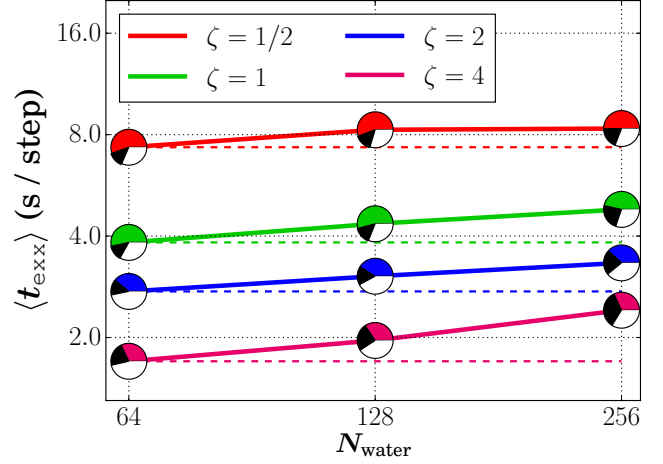
FIG. 9. Weak-scaling analysis of the MPI internode parallelization level in exx during CPMD simulations of liquid water at the hybrid PBE0 level on the Mira IBM Blue Gene/Q platform. For a fixed ratio of system size to number of processing elements ( i.e. , \zeta = 1/2 (red line), \zeta = 1 (green line), \zeta = 2 (blue line), and \zeta = 4 (magenta line)), the walltime spent in the exx module ( \langle t_{\text{exx}} \rangle in s/step, averaged over 50 CPMD steps) is plotted versus the system size, which was varied to include N_{\text{water}} = 64, 128, 256 water molecules. For reference, ideal weak-scaling timings were plotted as dashed lines for each \zeta , and were computed with respect to the corresponding (H_2O)_{64} timings. Pie plots were again used to illustrate the fraction of \langle t_{\text{exx}} \rangle dedicated to computation events ( f_{\text{exx}}^{\text{comp}} , colored), communication overhead ( f_{\text{exx}}^{\text{comm}} , black), and processor idling ( f_{\text{exx}}^{\text{idle}} , white).
