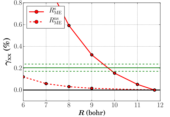
FIG. 7. Convergence of \{\tilde{D}_{\text{xx}}^i(\mathbf{r})\} (via the \gamma_{\text{xx}} metric defined in Eqs. (36) and (37)) as a function of R_{\text{ME}}^{\text{s}} and R_{\text{ME}}^{\text{ns}} on a snapshot of liquid water containing (\text{H}_2\text{O})_{64} in a cubic cell with L = 23.52 Bohr. Relative errors (in %) with respect to \{\tilde{D}_{\text{xx}}^{i,\text{ref}}(\mathbf{r})\} are evaluated by varying R_{\text{ME}}^{\text{s}} (solid red line) and R_{\text{ME}}^{\text{ns}} (dashed red line), while keeping all other parameters ( R_{\text{pair}} , R_{\text{PE}}^{\text{s}} , R_{\text{PE}}^{\text{ns}} ) set to their default values in QE (see text for more details). An overall relative error of \approx 0.2\% (with a standard deviation of \pm 0.03\% ) corresponds to the default parameter values in QE ( R_{\text{ME}}^{\text{s}} = 10.0 Bohr, R_{\text{ME}}^{\text{ns}} = 7.0 Bohr), and is depicted by the solid (dashed) green line.
