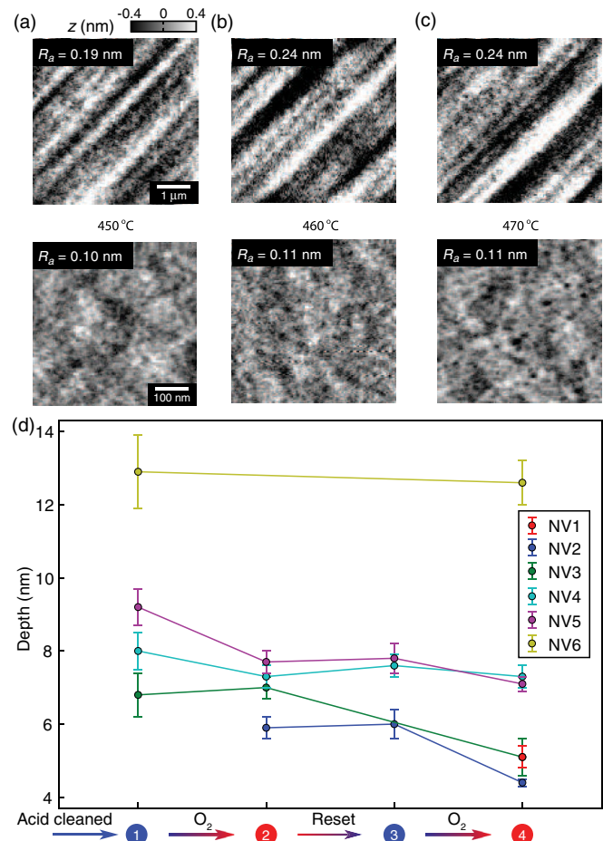
FIG. 7. (a)–(c) AFM images of a scaife-polished standard grade sample annealed at successively higher temperatures for temperature calibration of oxygen furnace. Micropits (black circles about 20 nm in diameter) are visible after the oxygen anneal at 470°C. (d) Depth measurements of the six NV centers presented in the main text after different annealing steps.
