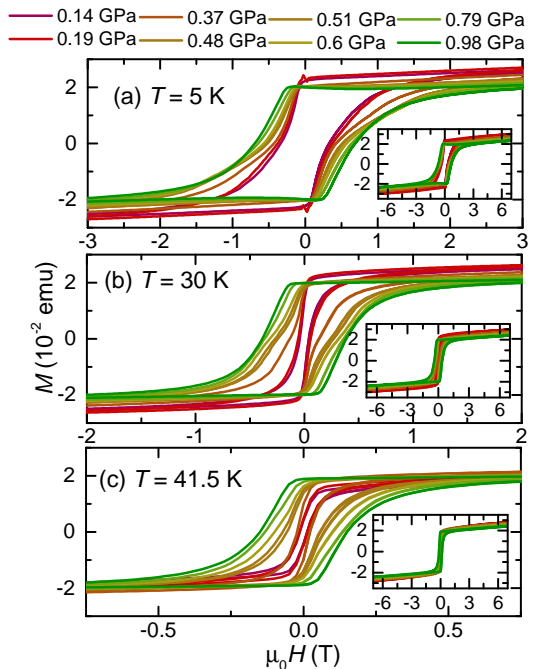
FIG. 10. Magnetization, M , vs. field, \mu_0 H , at T = 5 K (a), 30 K (b) and 41.5 K (c) at different pressures between 0.14 GPa and 0.98 GPa.
