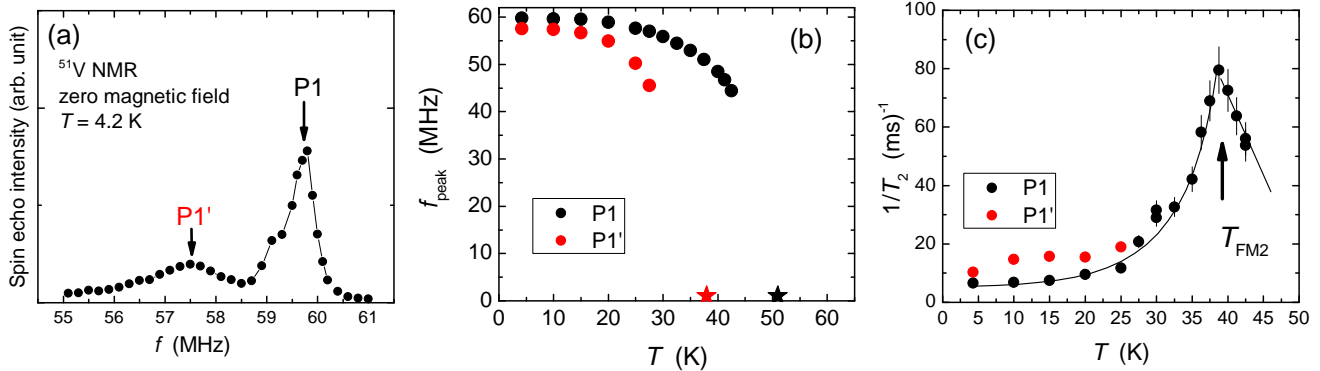
FIG. 4. (a) NMR spectrum in \text{VI}_3 measured at B = 0 T and T = 4.2 K at ambient pressure in the ferromagnetic state. The two peaks (labelled by P1 and P1') correspond to central transition lines of ^{51}\text{V} NMR. The ratio of the integrated intensities of P1 and P1' is estimated to be 1.7 : 1 after correction by their respective longitudinal and transverse relaxation times ( T_1 and T_2 , respectively); (b) Temperature dependence of f_{\text{peak}} for each peak at zero magnetic field. Black (red) star denotes the transition temperature T_{\text{FM2}} ( T_{\text{FM1}} ), inferred from specific heat and magnetization data in Fig. 2; (c) Temperature dependence of 1/T_2 for both P1 and P1' at zero magnetic field. 1/T_2 shows a peak at T \sim 38 K, which is very close to the second ferromagnetic phase transition temperature T_{\text{FM2}} , determined from magnetization and specific heat measurements. The solid curve is a guide to the eye.
