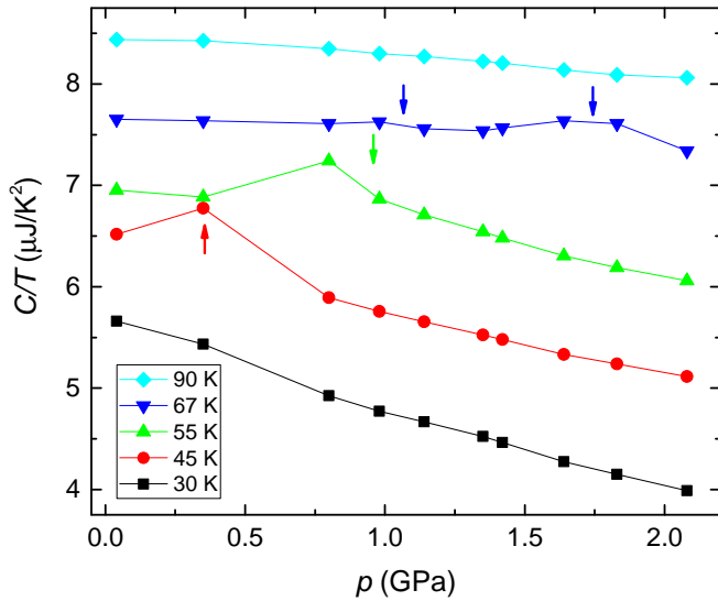
FIG. 9. Value of specific heat, C/T , vs. pressure, p at constant temperatures T = 30 \text{ K}, 45 \text{ K}, 55 \text{ K}, 67 \text{ K} and 90 \text{ K} . The arrows indicate the position of the various anomalies, associated with magnetic and structural transitions, in \text{VI}_3 under pressure (see main text for details). (Error for given pressure values is \Delta p \approx \pm 0.02 \text{ GPa} , i.e. smaller than the data points.)
