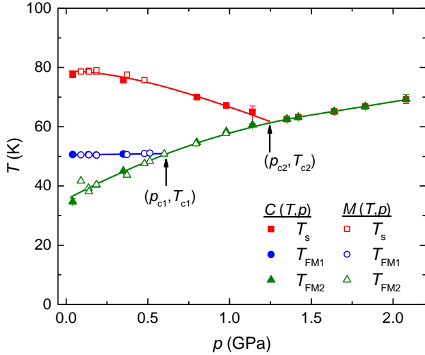
FIG. 8. Zero-field temperature ( T )-pressure ( p ) phase diagram of \text{VI}_3 , determined from specific heat measurements, C(T, p) (full symbols), and magnetization measurements, M(T, p) (open symbols). Squares denote the structural transition temperature T_s , circles the first ferromagnetic transition at T_{FM1} and triangulars the second ferromagnetic transition at T_{FM2} . The arrows mark the position of the two critical points in the phase diagram at (p_{c1}, T_{c1}) \approx (0.6 \text{ GPa}, 50.8 \text{ K}) and (p_{c2}, T_{c2}) \approx (1.25 \text{ GPa}, 61.6 \text{ K}) , which mark the merging of the two ferromagnetic transition lines and the ferromagnetic with the structural one, respectively. (Error for given pressure values is \Delta p \approx \pm 0.02 \text{ GPa} , i.e. smaller than the data points.)
