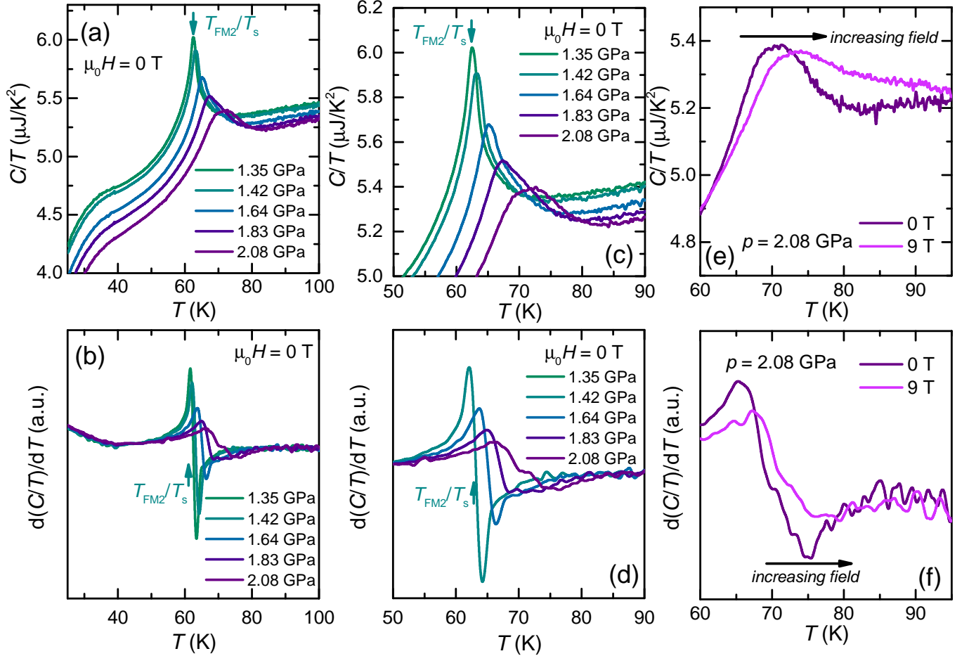
FIG. 7. Temperature-dependent specific heat, C/T , of \text{VI}_3 at different pressures for p \geq 1.35 GPa (Error for given pressure values is \Delta p \approx \pm 0.02 GPa.): (a) Specific heat data, taken in zero magnetic field. These data sets depict one anomaly (marked by the arrows for p = 1.35 GPa), which can be assigned to a simultaneous magnetic and structural transition at T_{FM2}/T_s ; (b) Temperature-derivative of the specific heat data, d(C/T)/dT , in (a). Arrows are used to visualize criteria to determine T_{FM2}/T_s for p = 1.3 GPa; (c,d) C/T and d(C/T)/dT , shown in (a) and (b), on enlarged scales; (e) Temperature-dependent specific heat, C/T , at p = 2.08 GPa in zero field and applied field ( \mu_0 H = 9 T); (f) Temperature-derivative of specific heat, d(C/T)/dT , at 0.8 GPa, 0.98 GPa and 1.14 GPa on enlarged scales around T_s (indicated by the arrows); (g) Temperature-derivative of the data shown in (e).
