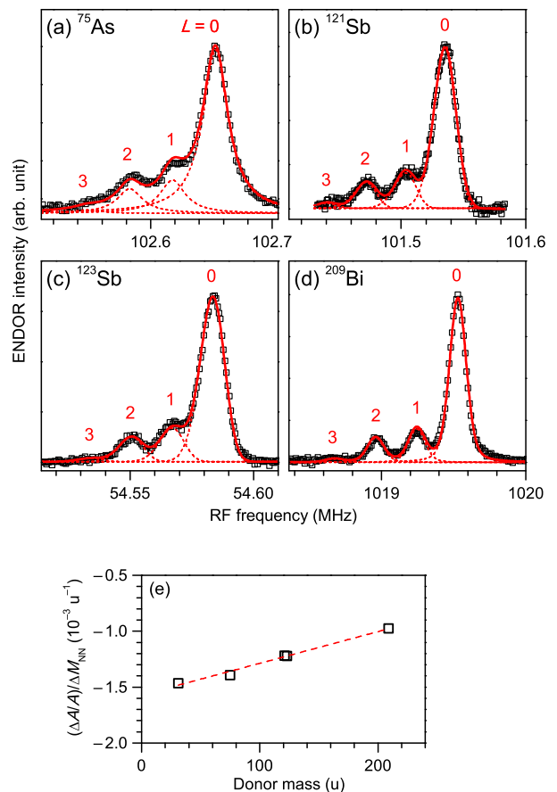
FIG. 3. (color online). The ENDOR spectra of (a) ^{75}\text{As} , (b) ^{121}\text{Sb} , (c) ^{123}\text{Sb} , and (d) ^{209}\text{Bi} donors in \text{natSi} . The open squares (black) are experimental data. The solid and dashed curves (red) are fitting results as employed in Fig. 2 with an optimized lineshape for all the components: asymmetric Lorentzian for (a), and asymmetric Gaussians for the other spectra. Each spectrum corresponds to the NMR transition of m_I = (-1/2 \rightarrow +1/2) , (-5/2 \rightarrow -3/2) , (-7/2 \rightarrow -5/2) , and (-7/2 \rightarrow -5/2) , respectively. The same labeling scheme L as in Fig. 2 is used to identify the peaks. (e) The fractional change of the hyperfine parameter with respect to M_{\text{NN}} (open squares) plotted as a function of the donor isotope mass along with a linear fit (dashed line) with a slope of 3 \times 10^{-6} \text{ u}^{-2} .
