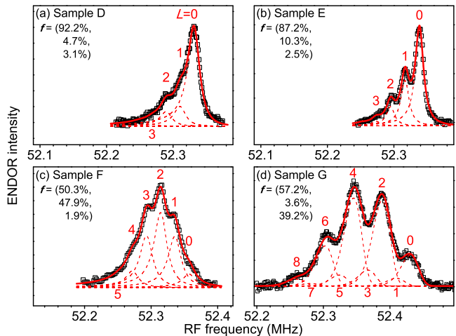
FIG. 2. (color online). Fitting of the ENDOR spectra for samples (a) D, (b) E, (c) F, and (d) G. The open squares (black) are experimental data. The solid and dashed curves (red) are fitting results of the full spectra and individual components ( L = 0 to 8), respectively. The relative intensities of the components are determined solely by the statistical probability of M_{\text{NN}} . The lineshape is optimized as common to all the components: asymmetric Gaussian for (d) and asymmetric Lorentzians for the rest. 38
