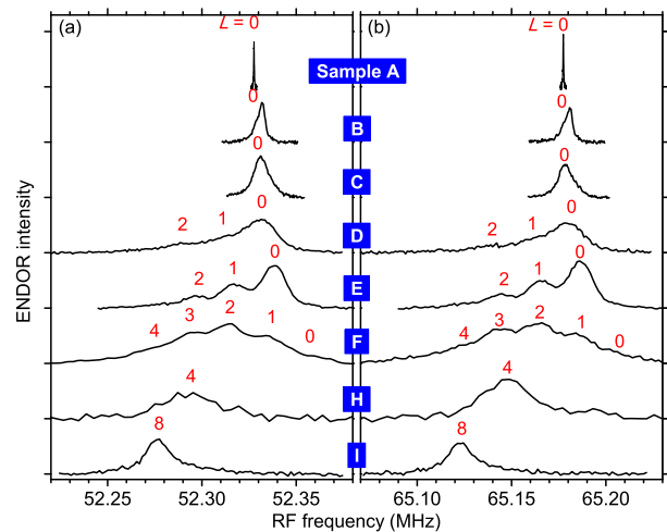
FIG. 1. (color online). 31 P ENDOR spectra of the (a) m_S = +1/2 and (b) m_S = -1/2 states for eight samples at the high-field (the nuclear spin projection m_I = -1/2 ) ESR line. M_{\text{bulk}} increases from top to bottom. A spectrum of G is shown independently in Fig. 2 (d) since it is too broad to fit in here and shifted slightly from others due to a small difference in the microwave excitation frequency employed in that particular measurement. Peaks are labeled with integers L = 0 to 8 based on the change in the average mass of the four NN Si isotopes, M_{\text{NN}} , as described later in the text.
