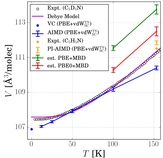
FIG. 2. Predicted and experimental thermal expansion curves for pyridine-I. Experimental data is included for pyridine-I ( C_5H_5N , gold circle), from single-crystal X-ray diffraction [40], and fully deuterated pyridine-I ( C_5D_5N , open black circles), from neutron powder diffraction [41]. A fit of the experimental thermal expansion curve for deuterated pyridine-I using the Debye model for V(T) is given by the purple line (Eq. (1)). Theoretical data is included for VC optimizations (blue circle), AIMD simulations (blue line), and PI-AIMD simulations (gold circle with error bar) at the PBE+vdW SC TS level; estimated PBE+MBD results (green line, Eq. (3)); estimated PBE0+MBD results (red line, see text for details).
