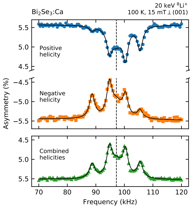
Figure 10. Typical helicity-resolved ^8\text{Li} spectra in BSC, revealing the fine structure of the line. Four quadrupole satellites, split asymmetrically in each helicity about a “central” Lorentzian (marked by a vertical dashed line) are evident. Note that, in contrast to conventional NMR, the satellite amplitudes are determined primarily by the highly polarized initial state. The solid black lines are the fits described in the text and the vertical dashed line marks the resonance central frequency \nu_0 .
