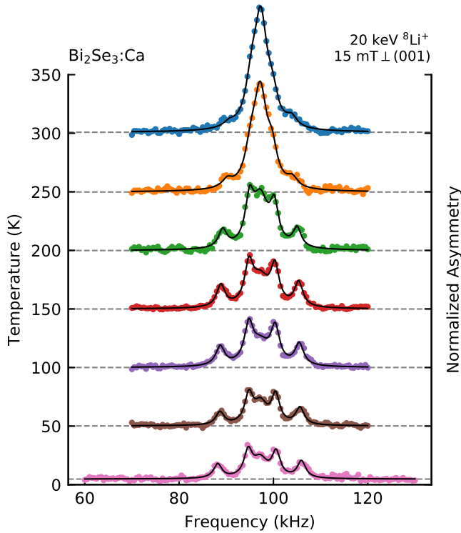
Figure 3. ^8\text{Li} resonance spectra in BSC at low magnetic field. The vertical scale is the same for all spectra; they have been normalized to account for changes in intensity due to SLR [41], with their baselines (shown as dashed grey lines) shifted to match the temperature. The spectra consist of a small and nearly temperature-independent quadrupole split pattern, centred about an unsplit Lorentzian line, whose amplitude grows above \sim 150 K. Note the quadrupole pattern of an integer spin nucleus like ^8\text{Li} , has no central satellite (main line). The solid black lines are fits to a sum of this Lorentzian plus and 2I = 4 quadrupole satellites (see text).
