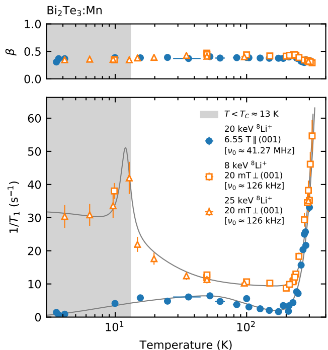
Figure 6. Temperature dependence of the ^8\text{Li} SLR rate 1/T_1 in Mn doped \text{Bi}_2\text{Te}_3 at high and low field. At low field, 1/T_1 shows a critical peak at the ferromagnetic transition at T_C \approx 13\text{ K} , as the Mn spin fluctuations freeze out. Above 200 K, the SLR rate increases exponentially in manner nearly independent of applied field. The solid grey lines are drawn to guide the eye.
