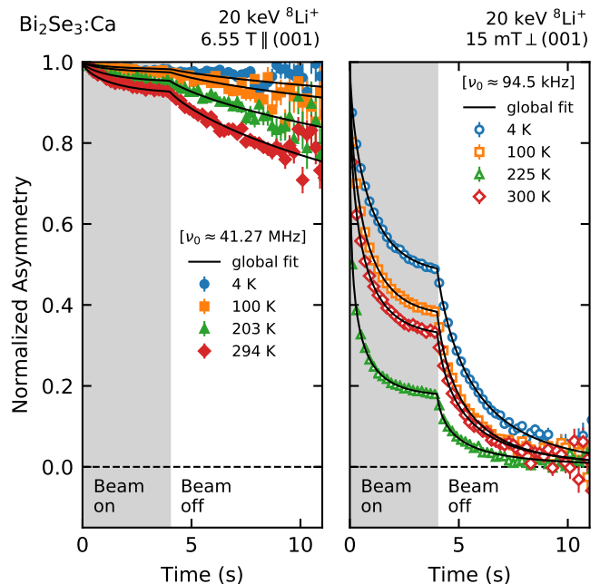
Figure 1. Typical ^8\text{Li} SLR spectra in Ca doped \text{Bi}_2\text{Se}_3 at high (left) and low (right) magnetic field with ^8\text{Li}^+ implanted at 20 keV. The shaded region indicates the duration of the ^8\text{Li}^+ beam pulse. The relaxation is strongly field dependent, increasing at lower fields, and it increases non-monotonically with increasing temperature. The solid black lines show fits to a stretched exponential described in the text. The initial asymmetry A_0 from the fits is used to normalize the data which are binned by a factor of 20 for clarity.
