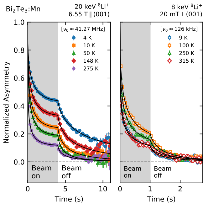
Figure 5. Typical ^8\text{Li} SLR spectra in Mn doped \text{Bi}_2\text{Te}_3 at high (left) and low (right) magnetic field for ^8\text{Li}^+ implantation energies of 20 keV and 8 keV, respectively. The shaded region denotes the duration of the ^8\text{Li}^+ beam pulse. The SLR is substantial and orders of magnitude faster than in BSC (see Figure 1) at high field. The field dependence to the SLR is much weaker than in the nonmagnetic tetradymites. The solid black lines are fits to a stretched exponential convoluted with the ^8\text{Li}^+ beam pulse as described in the text. The initial asymmetry A_0 from the fit is used to normalize the spectra. The high and low field spectra have been binned for by factors of 20 and 5, respectively.
