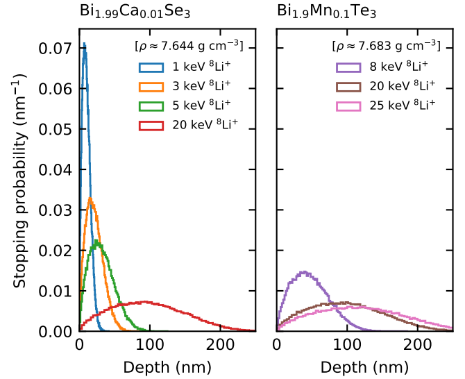
Figure 8. Stopping distribution for ^8\text{Li}^+ implanted in the doped TIs BSC and BTM, calculated using the SRIM Monte Carlo code [27] using 10^5 ions. The implanted probe ions stop principally within \sim 250 nm from the crystal surface, with only a minor “tail” penetrating further. Only at the lowest ^8\text{Li}^+ implantation energy 1 keV does an appreciable fraction ( \sim 15\% ) stop in the region where surface effects, are expected to be important.
