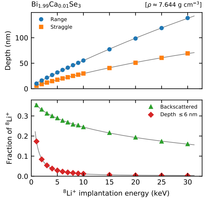
Figure 9. Stopping details for ^8\text{Li}^+ implanted in BSC calculated using the SRIM Monte Carlo code [27]. The ion stopping range and straggle (i.e., mean and standard deviation) at each implantation energy are shown in the top panel. The bottom panel shows the predicted fraction of ^8\text{Li}^+ that are backscattered and those that stop within the first \sim 6 nm, where surface effects are expected. Except at the lowest implantation energy, this latter fraction is negligible. The solid grey lines are drawn to guide the eye.
