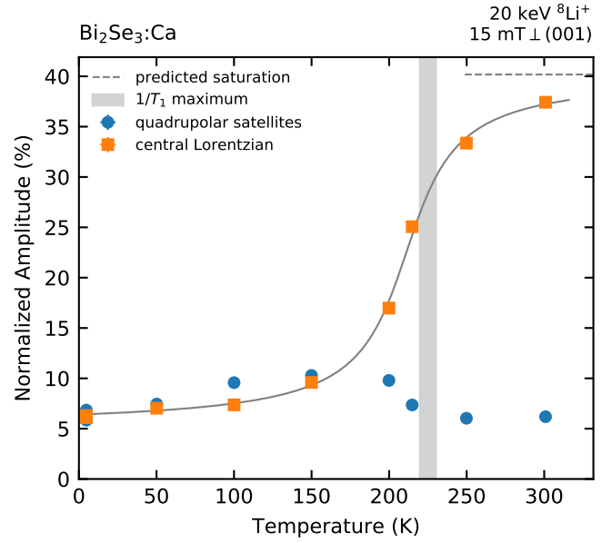
Figure 4. The resonance amplitude as a function of temperature in Ca doped \text{Bi}_2\text{Se}_3 at 15 mT. While the amplitude of the satellite lines are nearly temperature independent, the central component increases substantially above 150 K, plateauing on the high- T side of the 1/T_1 maximum (grey band). The solid line is a guide, while the dashed line indicates the estimated saturation value for the Lorentzian component.
