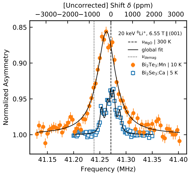
Figure 7. Typical ^8\text{Li} resonances in Mn doped \text{Bi}_2\text{Te}_3 and Ca doped \text{Bi}_2\text{Se}_3 at high magnetic field. The vertical scale is the same for both spectra; they have been normalized to account for changes in intensity and baseline [41]. The lineshape in the magnetic BTM is well-described by a broad Lorentzian (solid black line) with no quadrupolar splitting. A large negative shift is also apparent for BTM with respect to the reference frequency in MgO (vertical dashed line). The dotted vertical line indicates the expected resonance position due to demagnetization, revealing a large positive hyperfine field ( \sim 38 G) at 5 K in the magnetic state.
