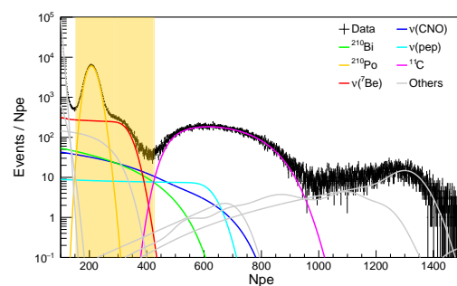
Figure 2: Borexino energy spectrum as a function of the energy estimator “geometry-normalized N_{pe} ”. Typical contribution to the spectrum in terms of solar neutrino electron scattering and \beta -like background are reported in the legend. The vertical yellow band shows the constant energy window region used for building up the time series of the total rate.
