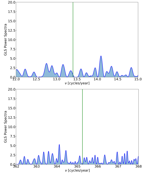
Figure 10: Top : A zoom-in of the GLS power spectrum (in arbitrary units) of the residual rate of Fig. 8 around the one cycle/month point. The Sun's synodic rotation line of 13.4 cycles/year is shown (green vertical line). Bottom : A zoom-in of GLS power spectrum (in arbitrary units) of the residual rate of Fig. 8 around the one cycle/day point. The Earth's rotation line of 365.2596 cycles/year is shown (green vertical line).
