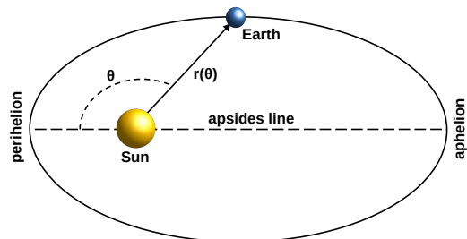
Figure 1: Earth's orbit around the Sun with parameters of interest. The Earth revolves around the Sun keeping the distance r(\theta) , where \theta is the angle with respect to the perihelion in polar coordinates. The eccentricity \epsilon is defined as the ratio between the difference and the sum of the aphelion and perihelion.
