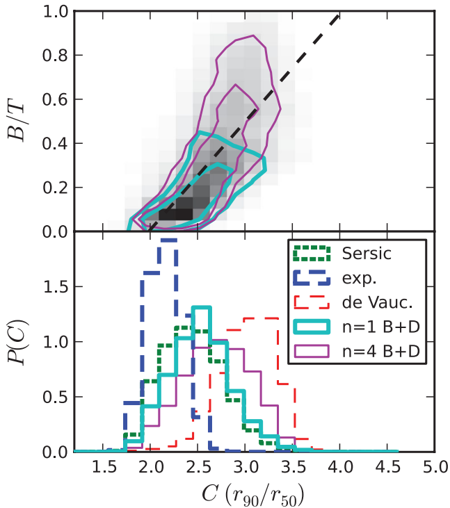
Figure 29. (Top): relation between B/T and Petrosian concentration for the sample of 20,726 B+D fitted galaxies. The underlying grey-scale map includes all galaxies, the thin magenta (thick cyan) contours show the n_b = 4(1) B+D modelled galaxies. The two contours in each colour enclose 50 and 80 percent of each sample. (Bottom): distributions of Petrosian concentration for the different categories of galaxies.
