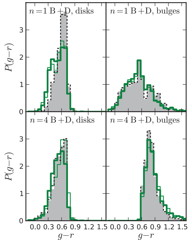
Figure 27. Same as Fig. 26, but for galaxies with intermediate inclinations ( 0.4 < q_d \leq 0.55 ).
