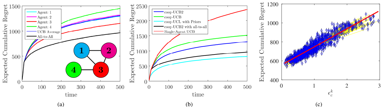
Fig. 1: (a) Simulation results comparing expected cumulative regret for different agents in the fixed network shown, using P as in (3) and \kappa = \frac{d_{\max}}{d_{\max}-1} . Note that agents 1 and 2 have nearly identical expected regret. (b) Simulation results of expected cumulative regret for several different MAB algorithms using the fixed network shown in Fig. 1(a). (c) Simulation results of expected cumulative regret as a function of normalized \epsilon_c^k for nodes in ER graphs at T = 500 . Also shown in red is the best linear fit.
