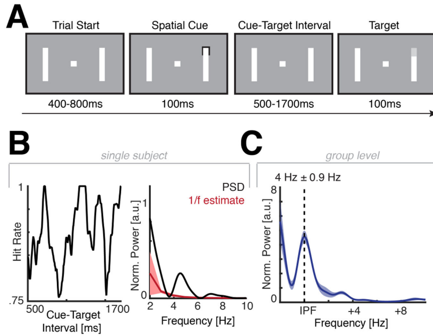
Figure 1. Task design and behavioral results of experiment 1
