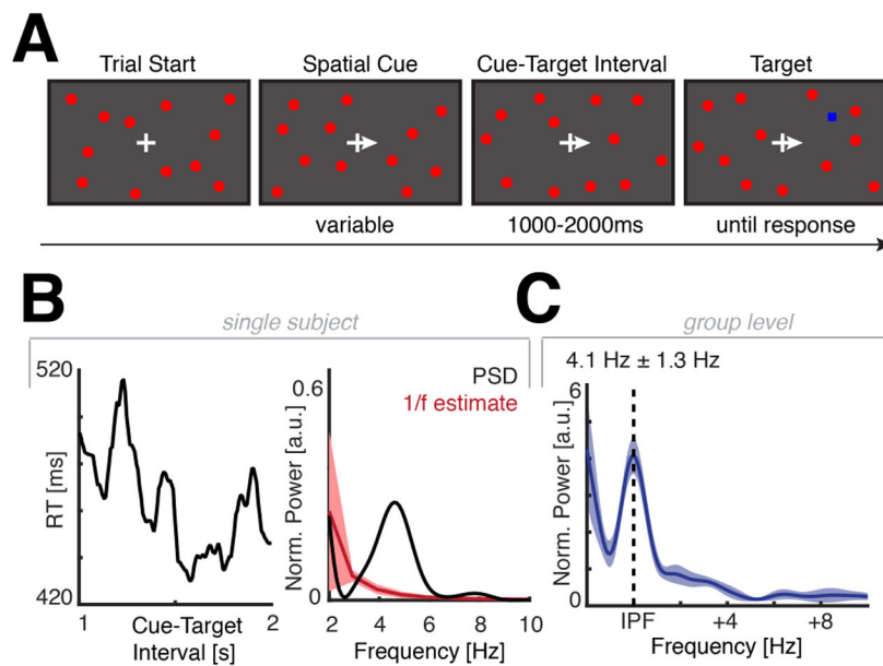
Figure 5. Task design and behavioral results of experiment 2
