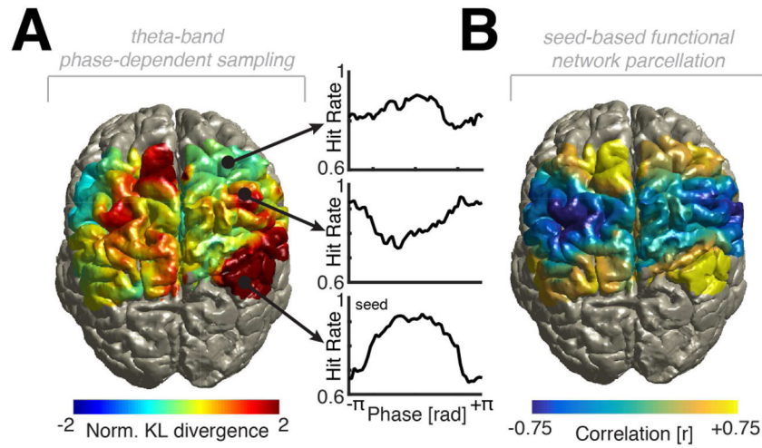
Figure 4. Large-scale network dynamics underlying rhythmic perceptual sampling (A) Left: Topographical depiction of rhythmic sampling in one example participant who was implanted with bilateral grids. Note that multiple regions contributed to the rhythmic sampling including frontal regions (upper right), sensorimotor regions (center right) and parietal regions (lower right). See Figure S5 for data from all participants. We seeded the electrode with the strongest phase-dependent behavioral modulation (lower right, located in IPS5). (B) Then we calculated seed-based correlations based on the phase-resolved behavioral data, which indicated that parietal and frontal areas exhibit the same preferred phase for optimal behavior.
