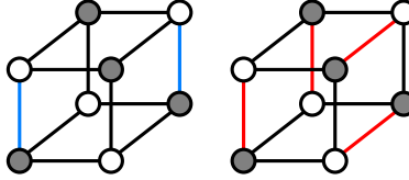
Figure 2: Hypercube on 8 nodes. Node shading represents the bipartition. On the left, the blue edges form an induced matching of size 2. On the right, the red edges form a matching of size 4 whose largest induced matching has size 1. Hence the multitasking capacity of the hypercube is at most 1/4 .
