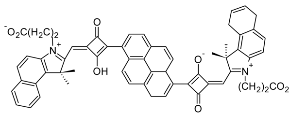
Fig. 11. Examples of squaraines (adapted from Umezawa 105 and Nakazumi 107 ).
