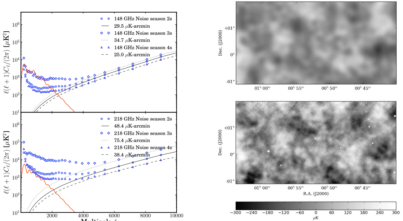
FIG. 5.— Comparison of a sky patch from the WMAP 7-year 94 GHz map (Jarosik et al. 2011) (top) with the map of the same region made from ACT 148 GHz (bottom) observations (co-added across seasons). All maps have been high-pass filtered with a \cos^2 \ell -like filter that goes from 0 to 1 for 100 < \ell < 300 . Agreement between the CMB features in the two maps is clear by eye.
