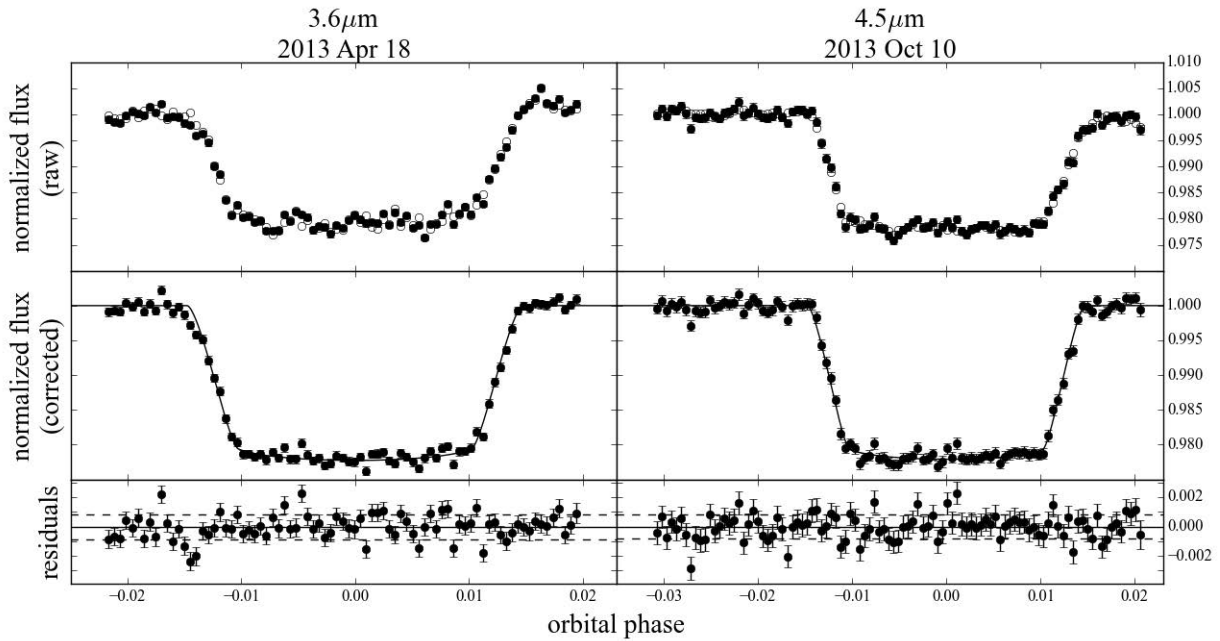
Figure 4. Spitzer IRAC 3.6- and 4.5- \mu\text{m} lightcurves for raw (top) and corrected (middle) white-light curves, where we have binned the data in time to three-minute intervals and divided out the best-fit instrumental noise model for each visit. Open circles in the top panel show the model points. The bottom panel shows the residuals after removing both the instrumental model and transit light curves. Error bars are the standard deviation of these residuals. Dashed lines show one standard deviation.
