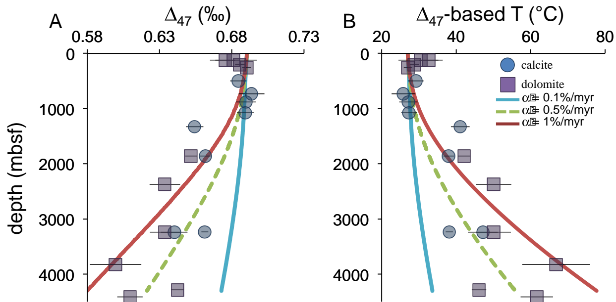
Figure 10: Comparison of the diagenetic model to data from a drill core through Andros Island, Bahamas. The data is from Winkelstern and Lohmann (2016). Models that use background recrystallization rates (a) of 0.5 to 1 %/myr follow the overall trends of the data. See section 7.2 for more details of the model. Error bars are 1 s.e.
