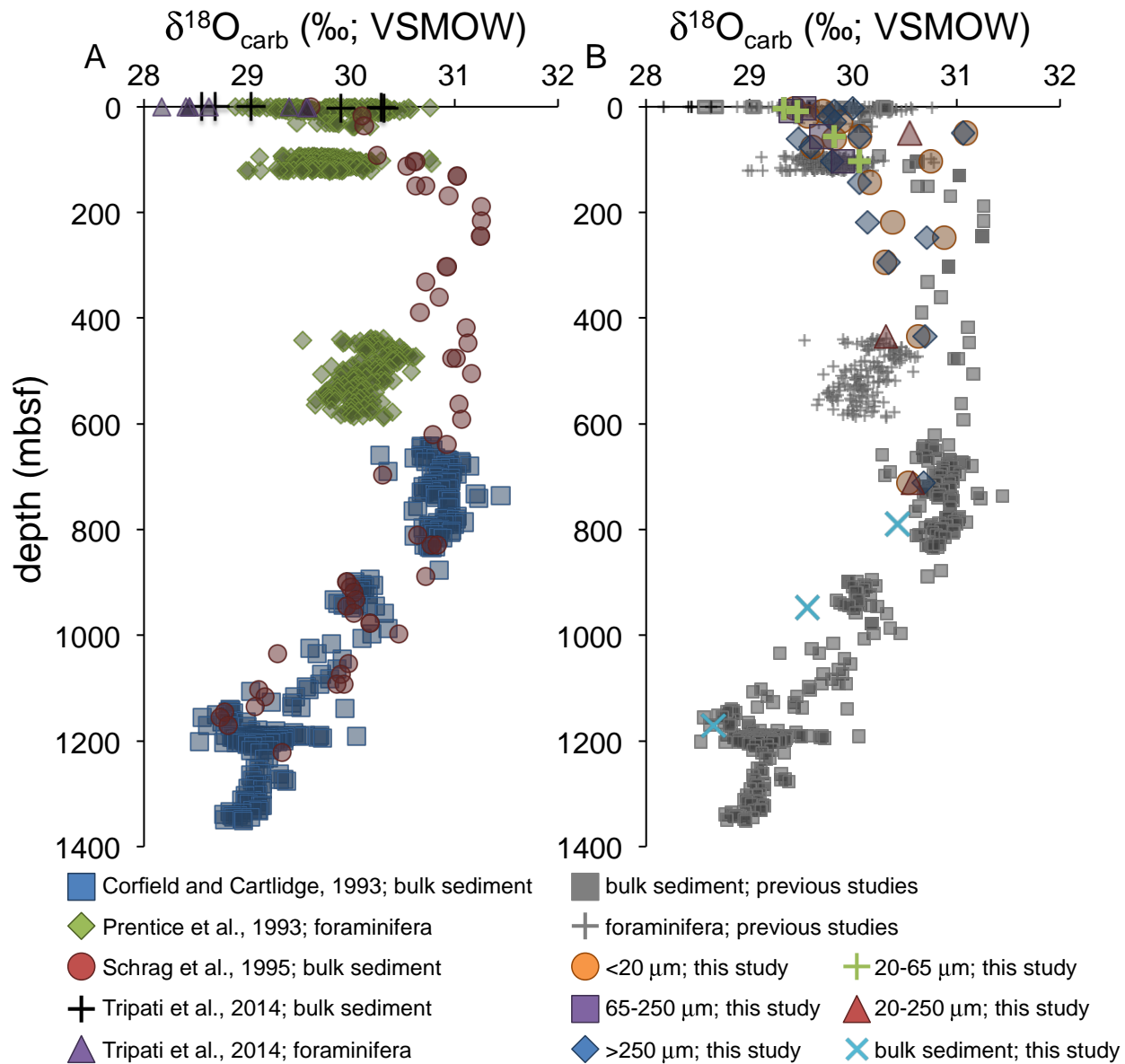
Figure 4: (A) Previously measured \delta^{18}\text{O}_{\text{carb}} values of bulk sediment and picked foraminifera from site 807 (Corfield and Cartlidge, 1993; Prentice et al., 1993; Schrag et al., 1995) and nearby sites (Tripati et al., 2014). (B) \delta^{18}\text{O}_{\text{carb}} values for various size fractions of carbonate sediments measured in this study and compared to previous measurements.
