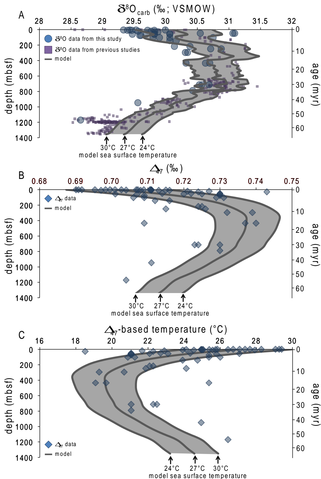
Figure 8: Comparison of the diagenetic model to site 807 data. For the model, we have assumed constant sea-surface temperatures of 24, 27, and 30°C, which are the range of temperatures observed for equatorial sea-surface temperatures in the area of study. Agreement between the model and data is apparent for samples <40 Ma (<800 m).
