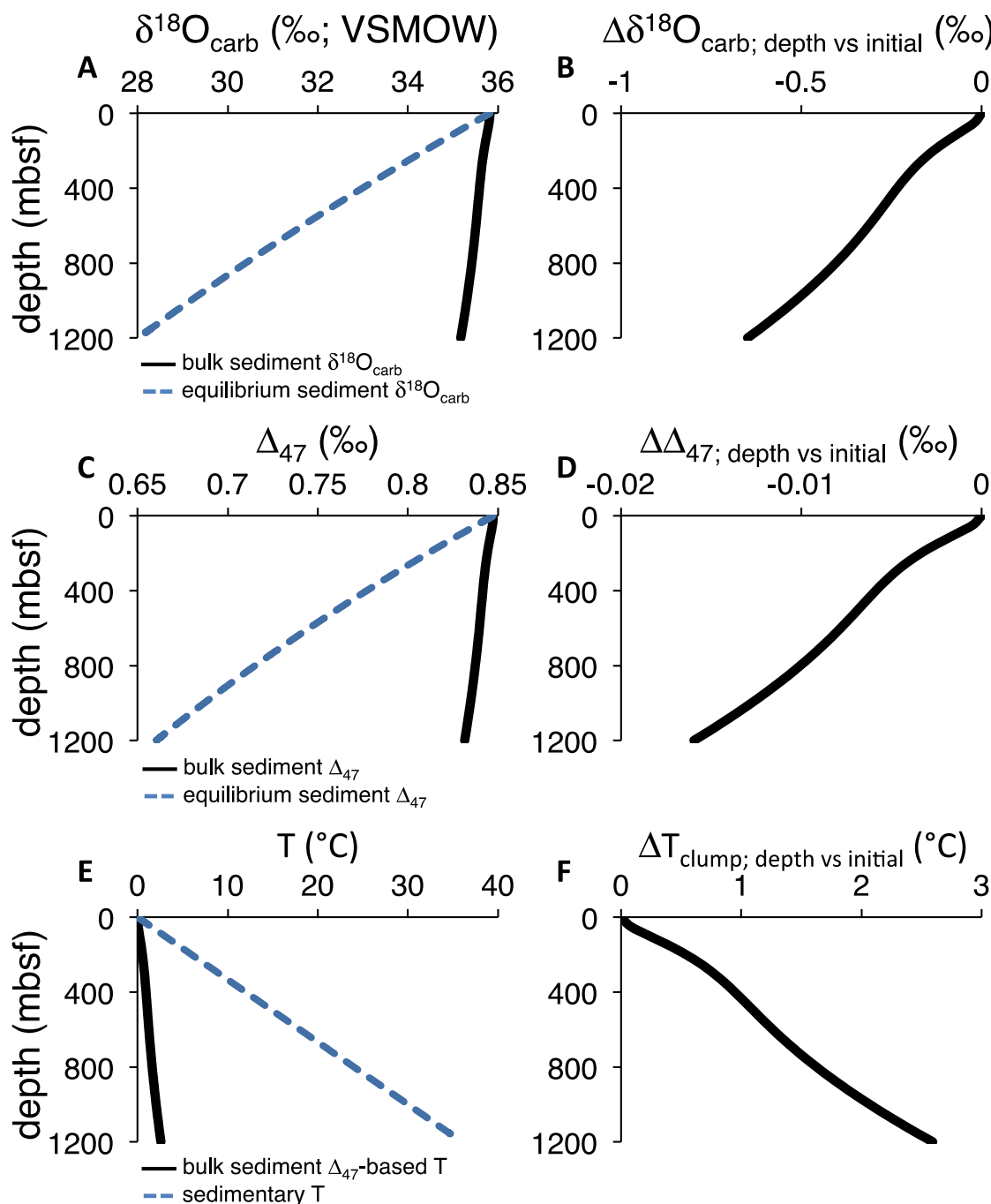
Figure 2: Model examples of the effects of dissolution-reprecipitation reactions on carbonate \delta^{18}\text{O}_{\text{carb}} , \Delta_{47} , and \Delta_{47} -based temperatures for a high-latitude deep-sea setting. Surface and deep-sea temperatures are 0°C. The geothermal gradient is 30 °C/km. \delta^{18}\text{O}_{\text{fluid}} value of seawater and the pore fluids are 0‰. Black lines are the bulk carbonate sediment values. Dashed blue lines are the values in the sediment column. In (B), (D), and (F) the change ( \Delta ) between the measured and initial value of the bulk carbonate as a function of depth is given. See section 3.1.4 for more details.
