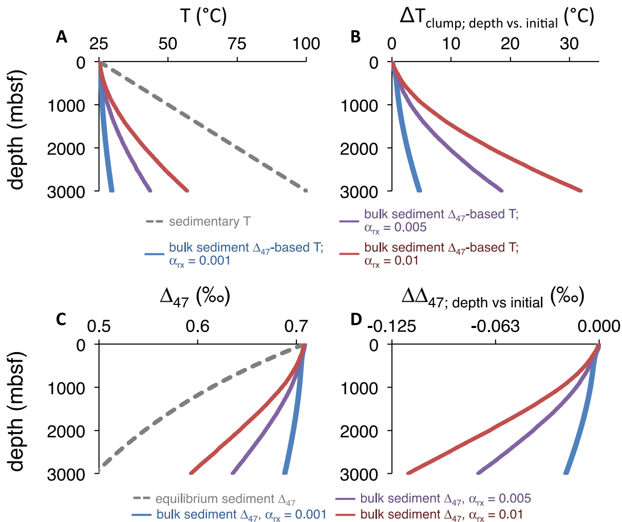
Figure 3: Model examples of the effects of dissolution-precipitation reactions on carbonate \Delta_{47} , and \Delta_{47} -based temperatures for a shallow sedimentary example. Surface and deep-sea temperatures are 25°C. The geothermal gradient is 25 °C/km. Dashed grey lines are the values in the sediment column. In (B), (D), the change ( \Delta ) between the measured and initial value of the bulk carbonate as a function of depth is given. \alpha_{rx} refers to the background reaction rate in the sedimentary column. See section 3.2.1 for more details
