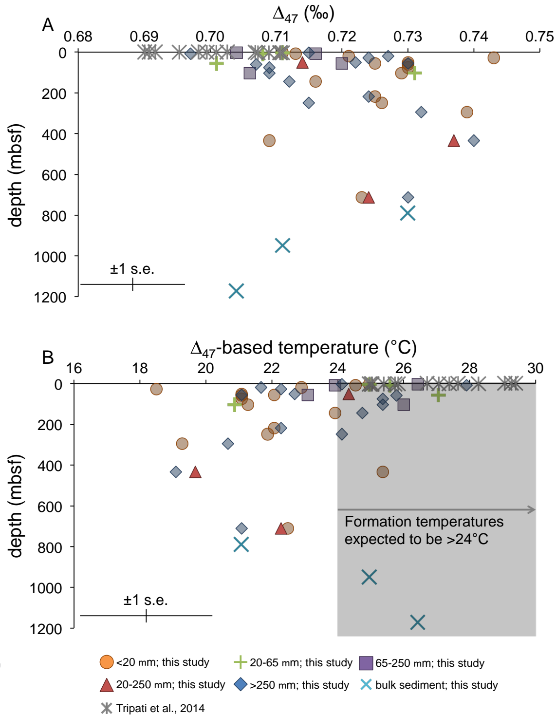
Figure 6: Clumped-isotope compositions and temperatures measured in this study and in Tripathi et al. (2014). (A) \Delta_{47} values vs. depth. (B) Measured \Delta_{47} -based temperatures. Based on previous reconstructions of equatorial sea-surface temperatures (Pearson et al., 2001; de Garidel-Thoron et al., 2005; Bijl et al., 2009; Kozdon et al., 2011; Zhang et al., 2014), original formation temperatures of all samples are expected to have been >24^{\circ}\text{C} . Therefore samples with \Delta_{47} -based temperatures <24^{\circ}\text{C} have likely been altered by diagenesis. Typical \pm 1 s.e. error bars are given for the \Delta_{47} measurements and \Delta_{47} -based temperatures.
