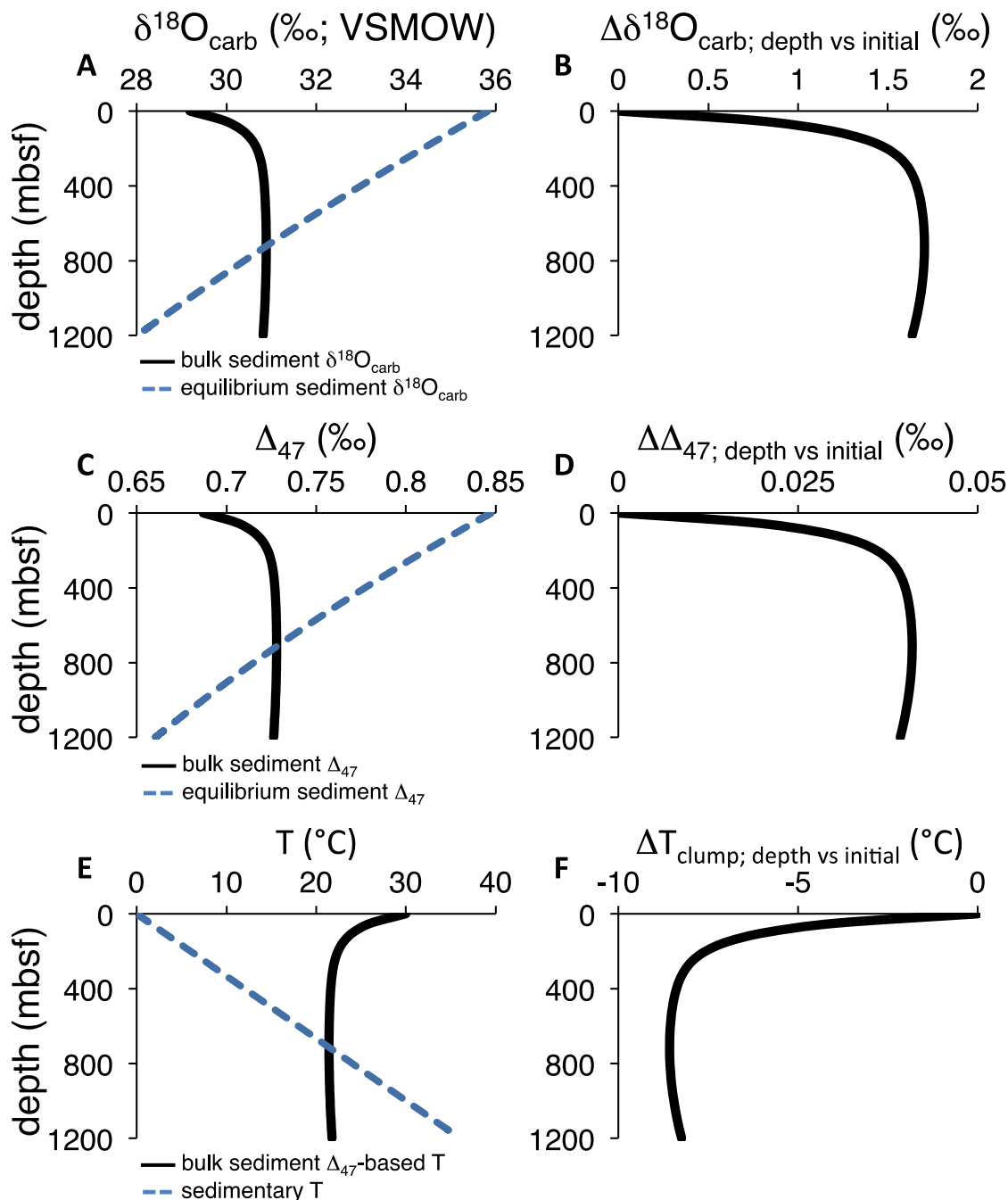
Figure 1: Model examples of the effects of dissolution-reprecipitation reactions on carbonate \delta^{18}\text{O}_{\text{carb}} , \Delta_{47} , and \Delta_{47} -based temperatures for an equatorial deep-sea setting. Surface temperatures are 30°C. Deep-water temperatures are 0°C. The geothermal gradient is 30 °C/km. \delta^{18}\text{O}_{\text{fluid}} value of seawater and the pore fluids are 0‰. Black lines are the bulk carbonate sediment values. Dashed blue lines are the values in the sediment column. In (B), (D), and (F) the change ( \Delta ) between the measured and initial value of the bulk carbonate as a function of depth is given. See section 3.1.4 for more details.
