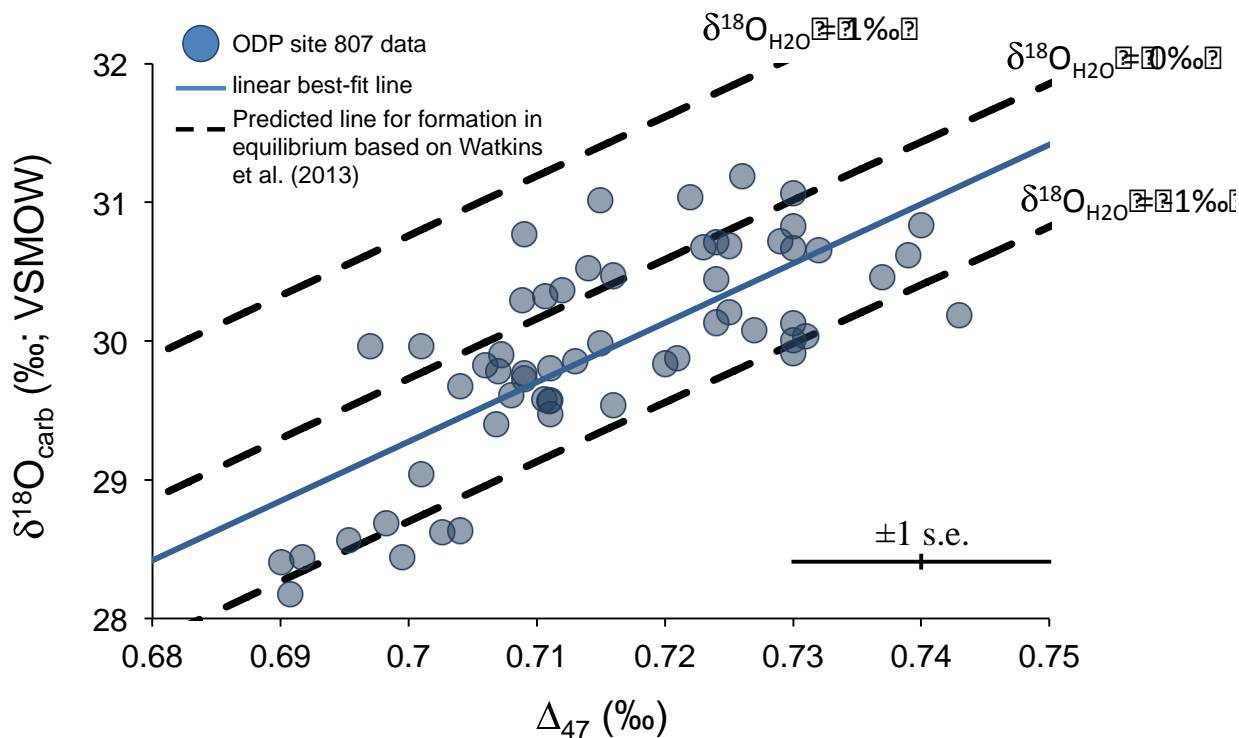
Figure 7: \delta^{18}\text{O}_{\text{carb}} vs. \Delta_{47} values. Lines for oxygen isotopic equilibrium between calcite and water for waters ranging from -1 to +1‰ (i.e., the ~range expected over the Cenozoic; Shackleton and Kennett, 1975; Miller et al., 1987; Adkins et al., 2002) are also given along with the best-fit line through the data. We note that points with \Delta_{47} values below 0.705‰ typically plot below the trend line. This is because these points are dominantly derived from picked foraminifera that precipitated their calcite with \delta^{18}\text{O} values lower than for measured bulk sediment (Tripathi et al., 2014).
