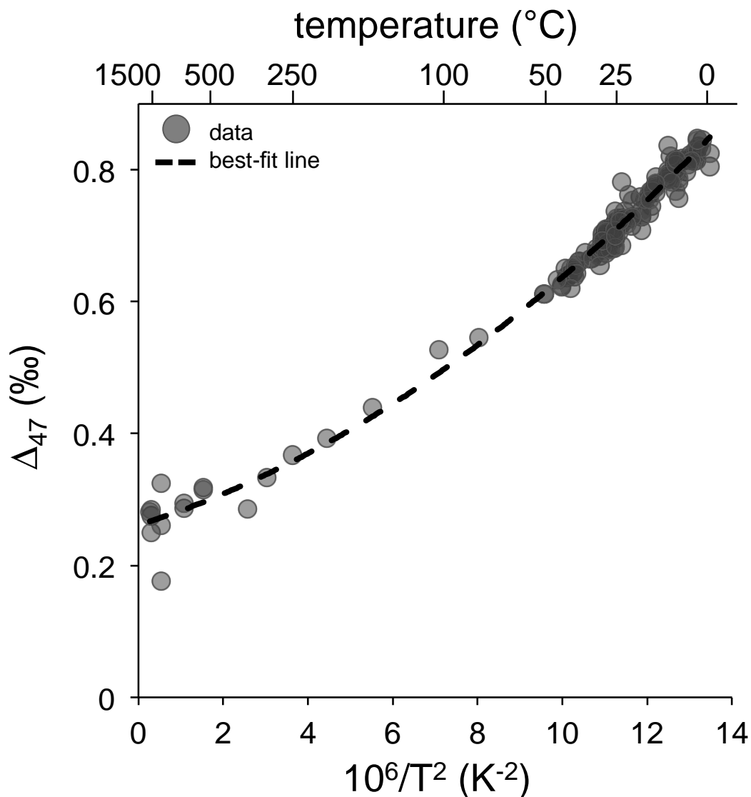
Figure A2: \Delta_{47} vs. temperature calibration used to simulate diagenesis at temperatures beyond 50°C, which is the highest temperature used in the Ghosh et al. (2006) calibration. This calibration was used solely in the model output presented in Figure 10. The equation is \Delta_{47} = 0.00173 \times (10^6/T^2)^2 + 0.0203 \times 10^6/T^2 + 0.261 where T is the temperature in Kelvin. Data used in this calibration comes only from measurement made at the Caltech laboratories (Ghosh et al., 2006; Ghosh et al., 2007; Came et al., 2007; Guo et al., 2009; Tripathi et al., 2010; Eagle et al., 2010; Thiagarajan et al., 2011; Dennis et al., 2011; Stolper and Eiler, 2015; Eagle et al., 2015; Spooner et al., 2016; Bonifacie et al., 2017).
