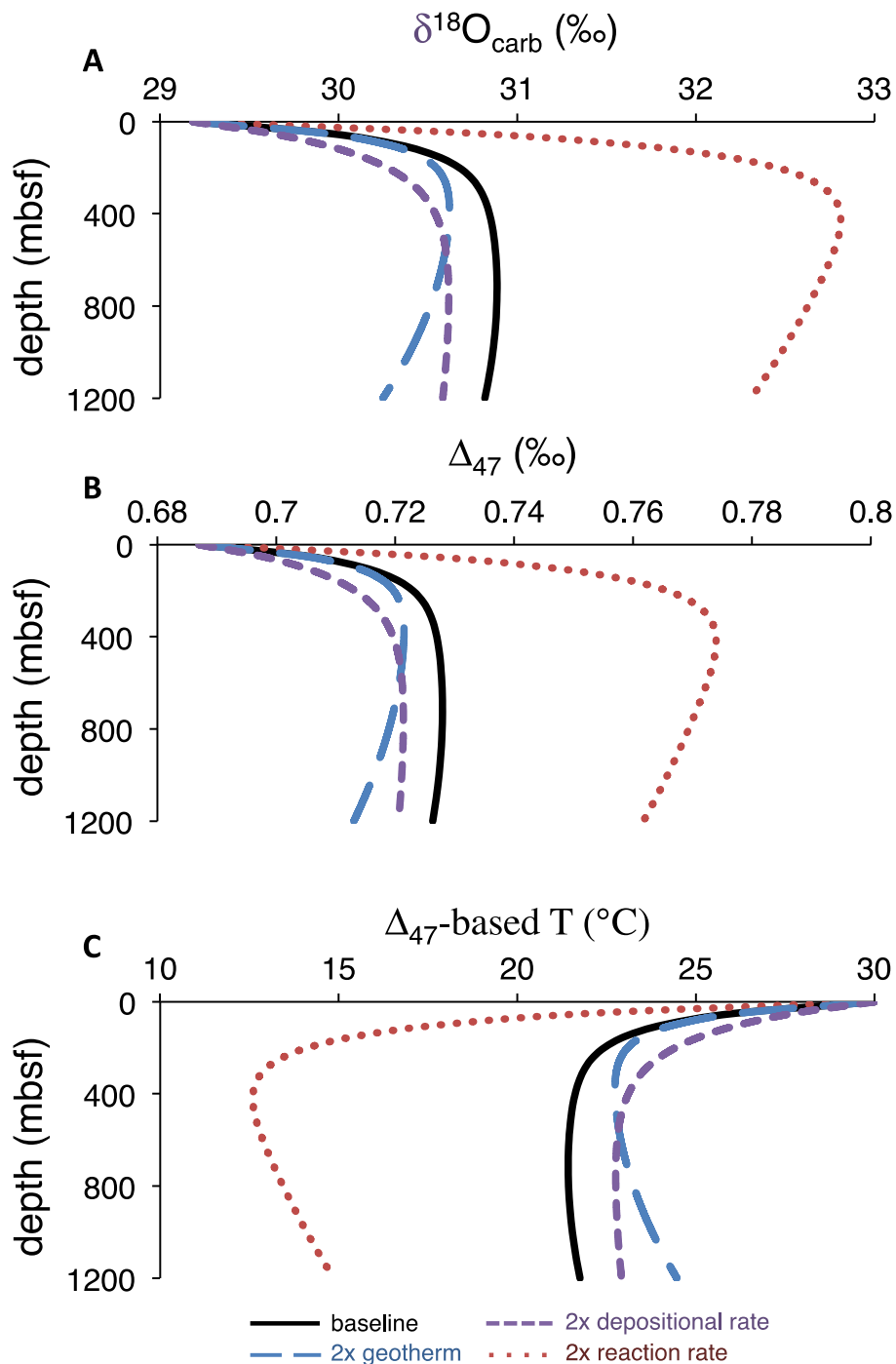
Figure A3: Comparison of changes in various model parameters including the geothermal gradient, depositional rate, and reaction rate on the effects of diagenesis on \delta^{18}\text{O} , \Delta_{47} values, and \Delta_{47} -based temperatures. The baseline model is the same as that given in Figure 2 (see section 3.1.4). When reaction rates are doubled (red line), we double \alpha_{\text{rx}} , \beta_{\text{rx}} , and \gamma_{\text{rx}} .
