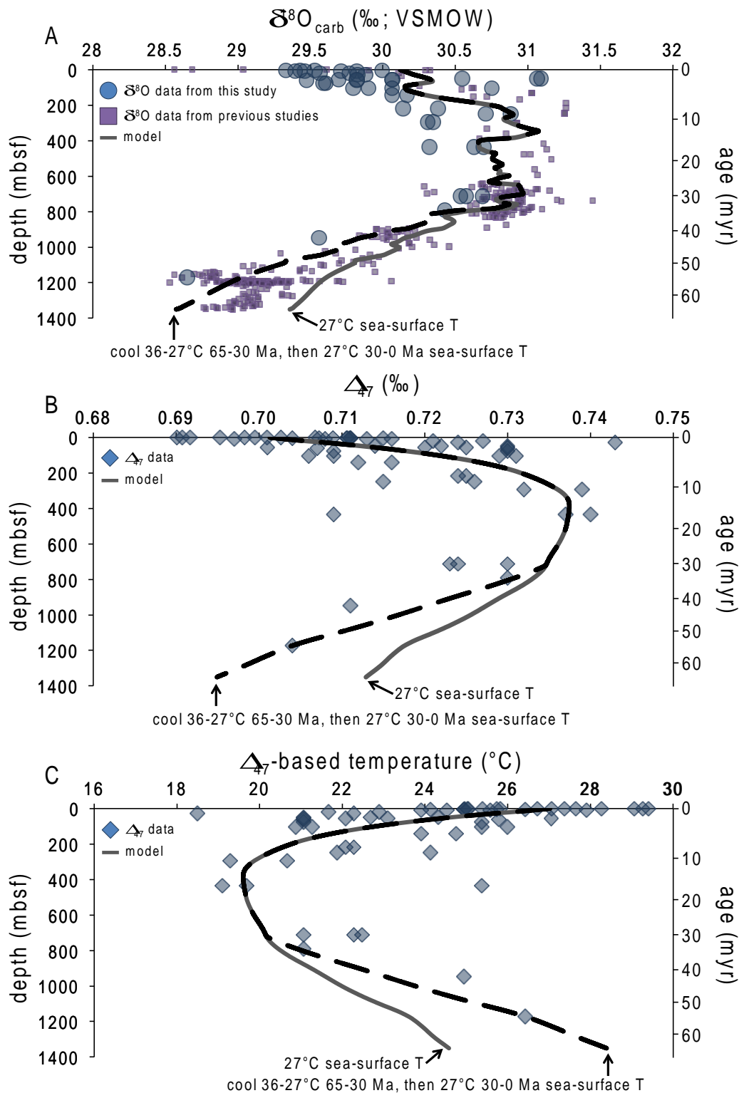
Figure 9: Comparison of the diagenetic model to site 807 data. Here we have compared a model in which sea-surface temperature are held at 27°C vs. a model where sea-surface temperatures cooled at a constant rate from 36 to 27°C from 65 to 30 Ma and then remained constant at 27°C until the present. Cooling over the course of the Paleogene provides a better fit to the data from 60-40 Ma.
