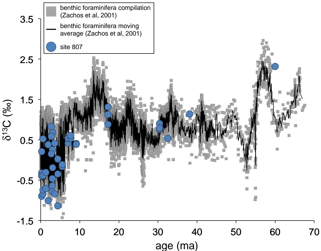
Figure 5: Site 807 carbonate \delta^{13}\text{C} values vs. those measured in other deep-sea cores for benthic foraminifera. Site 807 data are derived dominantly from planktonic organisms. To compare the two records, we lowered site 807 \delta^{13}\text{C} values by 0.95‰, which is the current difference in \delta^{13}\text{C} between surface and deep water values in the western Pacific Ocean (Kroopnick, 1985). Sediment age are derived from the age model given in Kroenke et al. (1991)
