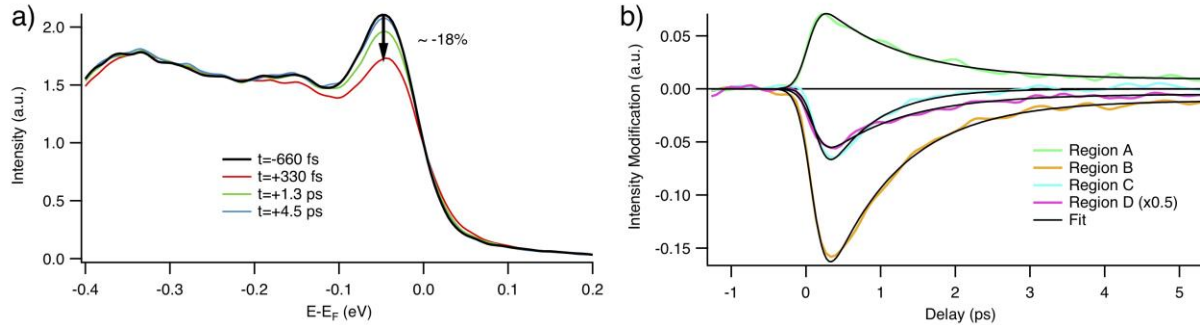
Fig. 7: Non-equilibrium dynamics. (a) Energy distribution curves collected at t=-660 fs, t=+330 fs, t=+1.3 ps, t=+4.5 ps. (b) Electron dynamics extracted at selected energy-momentum windows, as indicated in Fig. 6c. The solid black lines are fit to the data of an exponentially decaying function.
