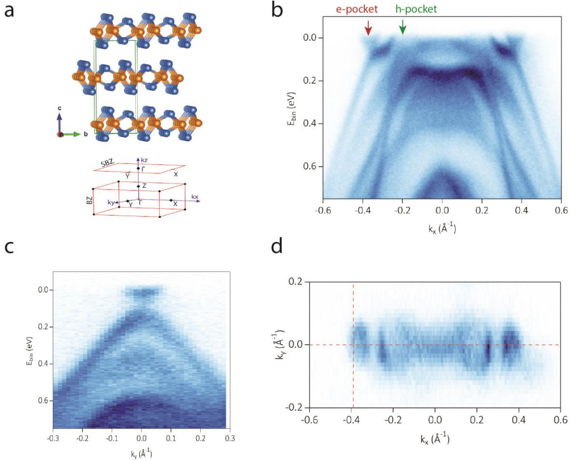
Fig. 1: Electronic structure of WTe_2 measured by ARPES. (a) Crystal structure of WTe_2 . A layer of W atoms is sandwiched between two Te layers. Then each di-chalcogenide layers are stacked along the crystallographic c -direction and bonded by weak van der Waals coupling. Bottom of the panel a) shows the Brillouin zone and surface Brillouin zone in reciprocal space. (b) band dispersion of WTe_2 measured by high resolution ARPES along the X - \Gamma - X direction which is the direction of the Te-W-Te chains. Well defined electron and hole pockets are observed on both sides of the Brillouin zone center ( \Gamma ) as marked by the red and green arrows (shown only on one side), respectively. Panel (c) shows the band dispersion along the Y - \Gamma - Y direction. (d) the Fermi surface map is shown with the dotted lines marking the band cuts shown in panel b and c, respectively.
