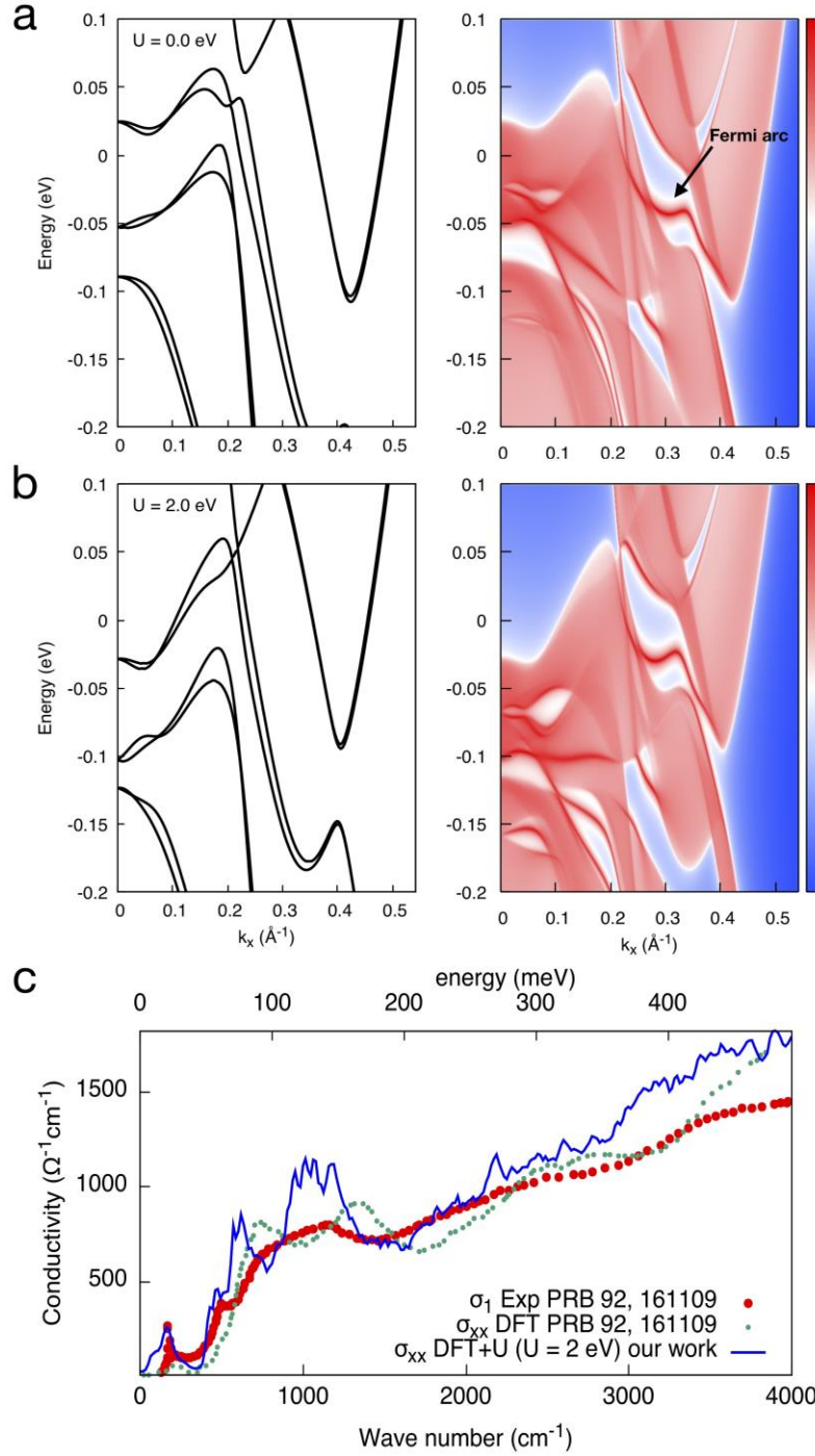
Fig. 5: (a-b) DFT+U band structure along the k_x direction (left panels) and corresponding theoretical spectral function for the (001) surface (right panel) as calculated for (a) U = 0.0 eV and (b) U = 2.0 eV. In the spectral function shown in panel (a) the black arrow highlights the Fermi arc which connects the hole and electron pockets in a type-II Weyl semimetal. (c) The experimental optical conductivity (red dots) is compared with the theoretical optical conductivity calculated by setting U = 0.0 eV (green dots) and U = 2.0 eV (blue solid line).
