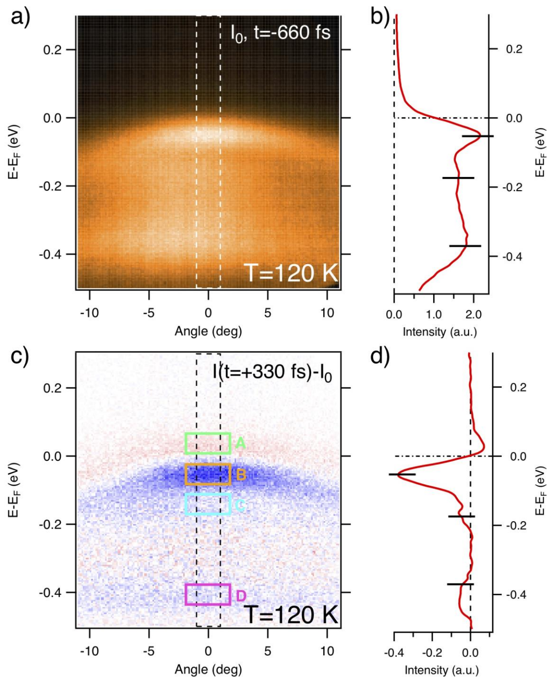
Fig. 6: Non-Equilibrium Electronic Structure by TR-ARPES Experiments. (a) The electronic band structure along \Gamma - Y direction ( k_x=0 ), measured at h\nu=6.2 eV and T=120 K. The map has been acquired at t=-660 fs. (b) Energy-distribution curve integrated in a \pm 1 degree window centered about k_y=0 (white dashed rectangle in panel a). Three main structures, in agreement with findings
