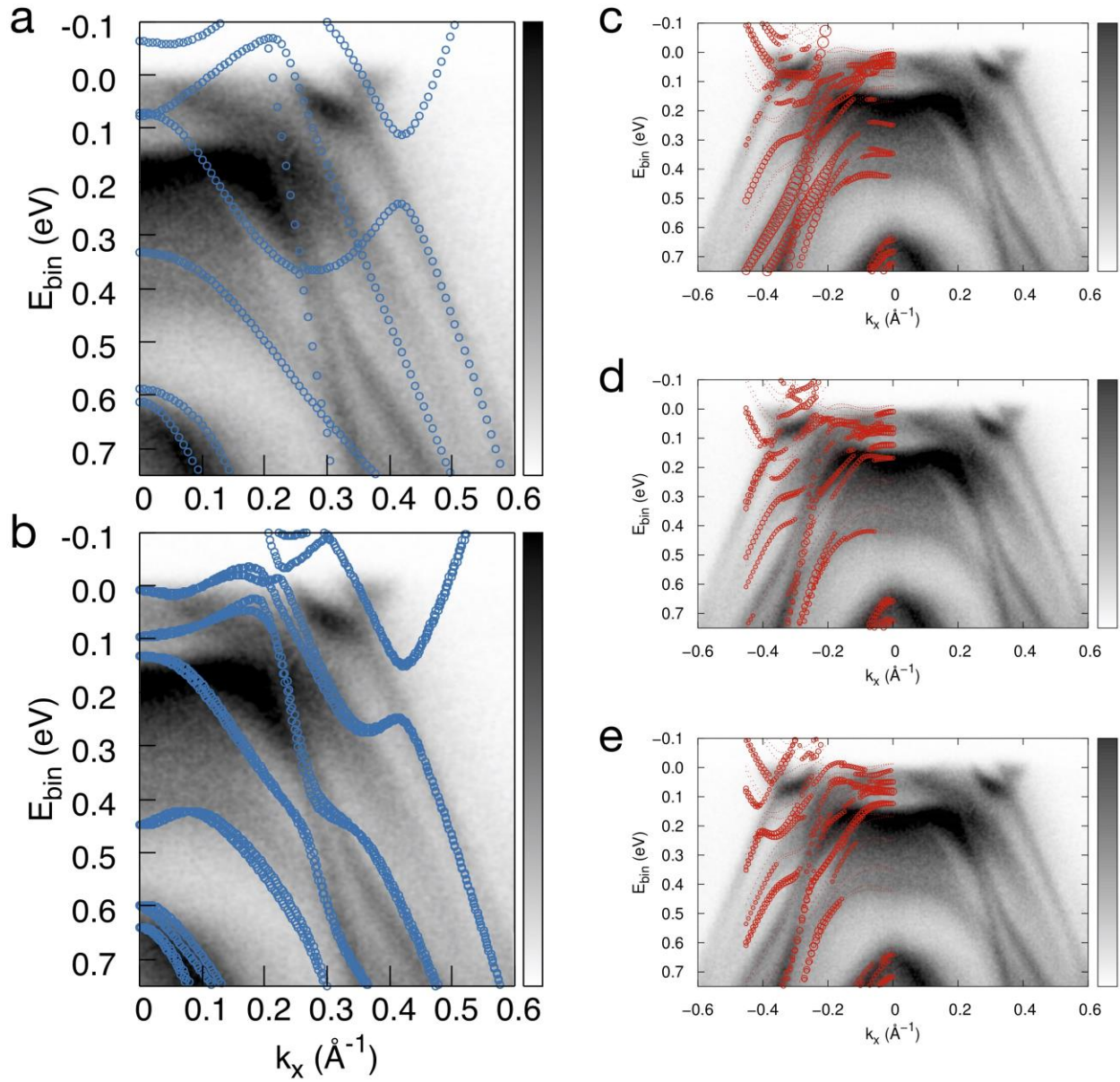
Fig. 2: (a-b) Bulk electronic band structure (blue symbols) as calculated without and with the inclusion of SOC, respectively, superimposed to the UV-ARPES measurements ( h\nu = 68 eV, T = 77 K) along the k_x direction, i.e. along the W zigzag chains. (c-e) Band structure (red symbols) of a \text{WTe}_2 finite slab projected onto the 1 th , 2 nd and 3 rd \text{WTe}_2 plane, respectively, superimposed to the same UV-ARPES spectrum as in panels (a-b).
