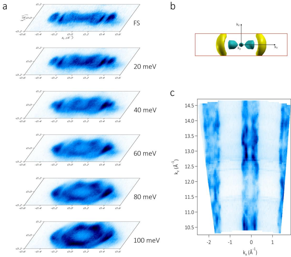
Fig. 3: Details of the Fermi volume. (a) Iso-energy k_x vs k_y cuts at the Fermi energy and each 20 meV below down to 100 meV binding energy. (b) simulated k_x vs k_z dispersion, and (c) k_x vs k_z Fermi surface as measured by soft-X-ray ARPES by changing the probe energy from 400 eV to 800 eV.
