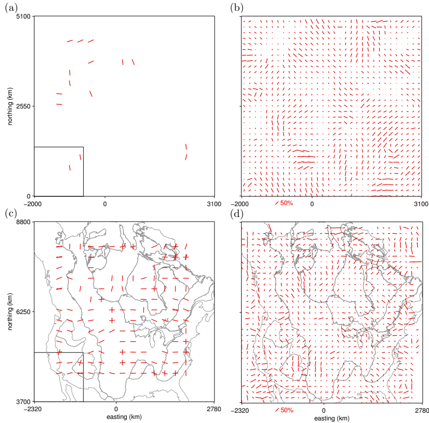
Figure 3: Testing coherence and elastic thickness estimates for mathematically significant anisotropy: synthetic data example. Directions show maxima in the coherence, which correspond to minima in T_e . (a) and (b) show results using Simons and Olhede (2013) synthetics analysed using multitaper and fan-wavelet methods, respectively. (c) and (d) show the corresponding results for the Kirby and Swain (2009) synthetics. For the multitaper method, results are shown after mathematical significance testing, and the window size of 1400 km is shown in the lower left. In the fan-wavelet results, the spatial domain of signal extraction scales inversely with the wavenumber and the length of the bars is scaled to the purported strength of the lithospheric anisotropy. All of the anisotropy is spurious. Of the anisotropy in (a) and (c), 100% of that in (a) and 89% of that in (c) is later identified and removed by the geophysical significance and topography/gravity bias tests.
