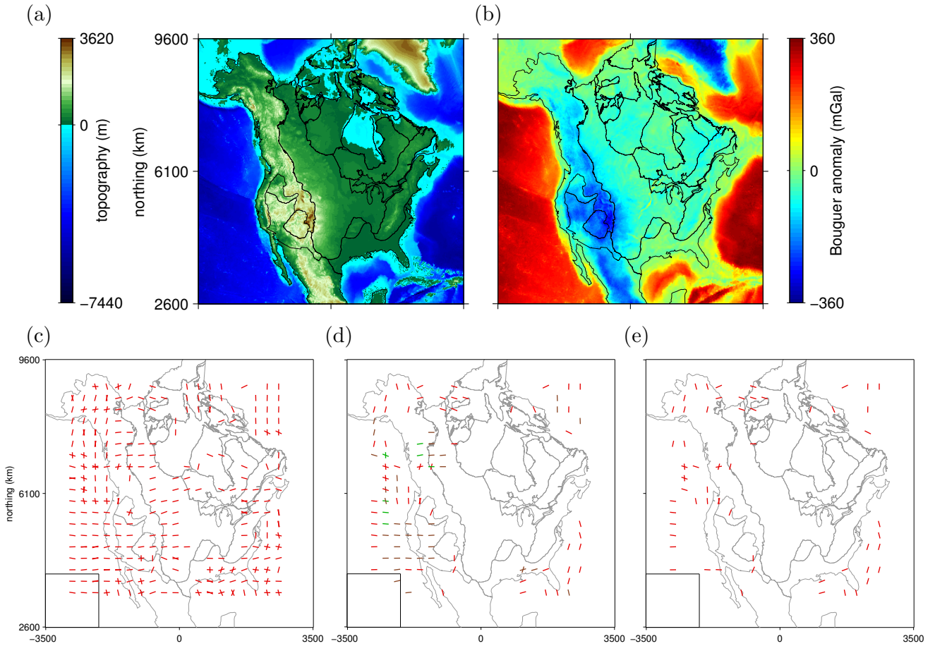
Figure 4: North American topography, gravity, and mechanical anisotropy from directional coherence analysis. (a) Topography and (b) Bouguer gravity anomaly from the EGM2008 model (Pavlis et al., 2012); the Bouguer anomaly is calculated from the model using the infinite-slab method with a crustal density of 2670 \text{ kg/m}^3 and a mantle density of 3300 \text{ kg/m}^3 . (c) Mathematically significant weak directions detected with a square window size of 1400 km. (d) Weak directions surviving mathematical and geophysical significance testing. Directions aligned with gravity or topography are shown in green or brown, respectively. (e) Weak directions surviving mathematical, geophysical, and bias testing.
