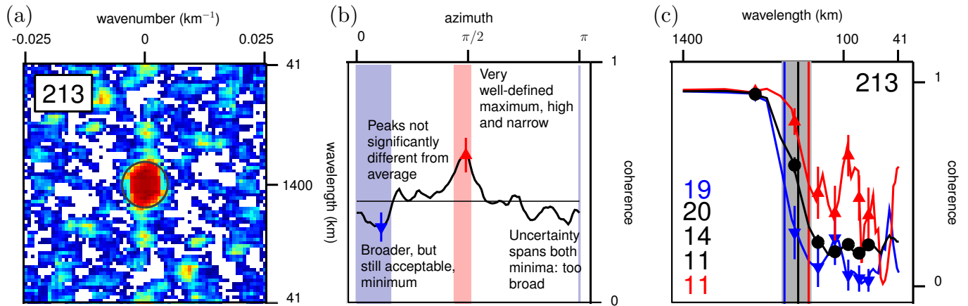
Figure 1: Testing coherence and elastic thickness estimates for anisotropy: real data example. All error bars shown are plus/minus two standard deviations. (a) An example with visible anisotropy in the north-south direction. The azimuthally averaged coherence reaches 0.5 at a wavelength of 213 km, marked by the black circle. Values below 0.1 left white. (b) Mean coherence (averaged over azimuth and wavenumber; horizontal black line), and radially averaged coherence (a function of azimuth; thick black curve), with red and blue triangles indicating the global maximum and minimum. Shading defines ranges of significant and well-resolved anisotropy, in this case around one directional low (blue) and one high (red) in the coherence. (c) Azimuthally averaged coherence (a function of wavenumber; black), with filled symbols showing approximately statistically uncorrelated wavenumbers. Coherence in the directions of the maximum (red), and minimum radially averaged coherence (blue). Vertical lines mark the half-points of the curves. Grey band marks the wavenumber uncertainty of the azimuthally averaged (black) half-points. As in (a), 213 is the wavelength of the half-point. The directional T_e estimates are 19 km (from the blue curve) and 11 km (from the red curve). The T_e estimate from the isotropic average (black curve) is 14 km with lower and upper bounds of 11 km and 20 km. As the isotropic bounds exceed the directional estimates, there is no robust indication of anisotropy in the effective elastic thickness.
