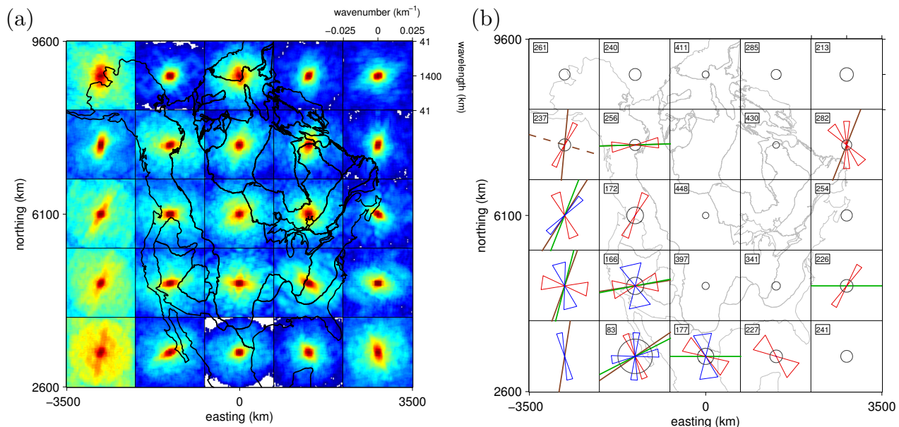
Figure 2: Possible bias in the coherence anisotropy from topography or gravity anisotropy and summary of the continent-wide analysis for mechanical anisotropy. (a) Power spectral density of North American topography from the EGM208 model (Pavlis et al., 2012), analysed in 1400 \times 1400 km non-overlapping patches. Geological province boundaries are after Vigil et al. (2000). (b) Mechanical anisotropy in the North American lithosphere analysed from topography and Bouguer gravity over the same 25 windows shown in (a). Black circles identify azimuthally-averaged coherence half-points, and boxed numbers their corresponding wavelengths in km, as in Figure 1a. Red and blue wedges show azimuthal ranges of (high and low, respectively) coherence anisotropy that pass both the mathematical (Figure 1b) and geophysical (Figure 1c) significance tests. Brown and green lines indicate significant maxima (solid lines) and minima (dashed lines) in the radially averaged power spectral density of the topography and Bouguer gravity anomaly, respectively. No values or measurements are plotted when the measurements are deemed insufficiently well determined.
