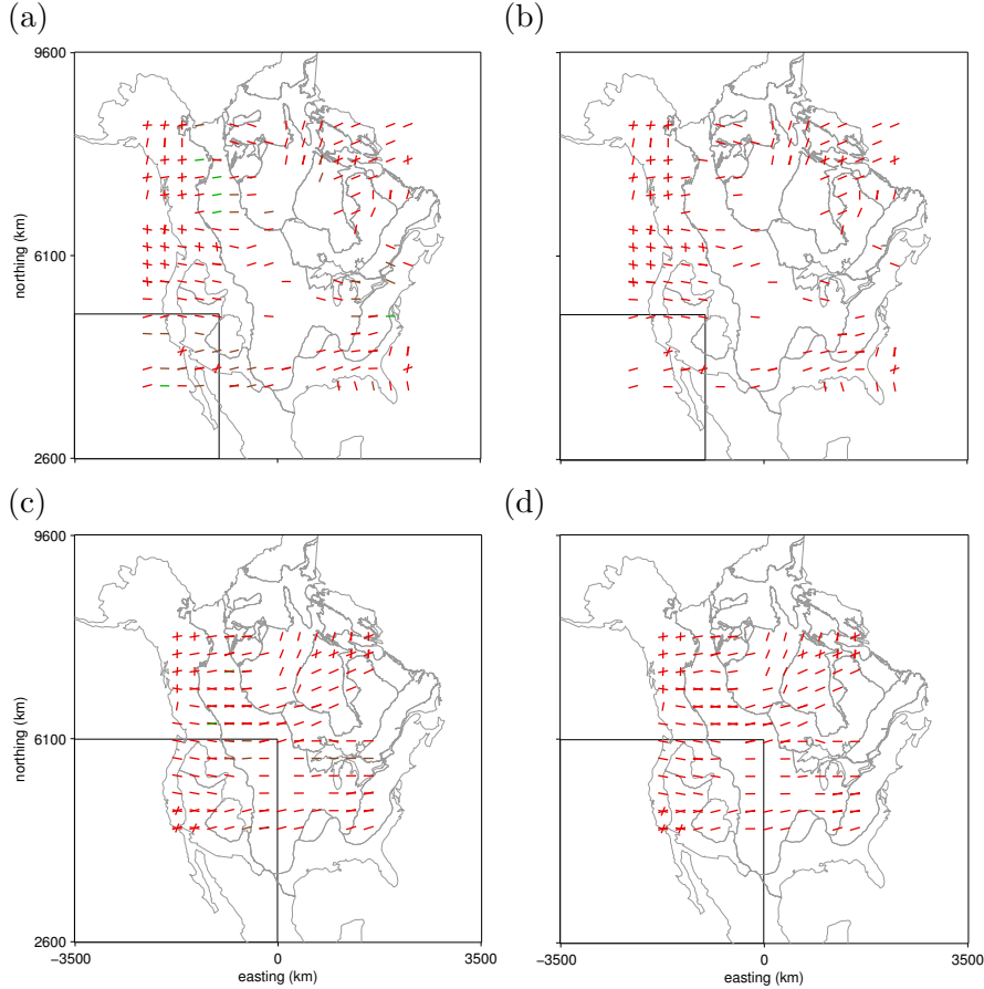
Figure 5: Weak directions surviving mathematical and geophysical significance testing (a and c) and all three tests (b and d), as in Fig. 4d and e, respectively, but with window sizes of (a–b) 2500 km and (c–d) 3500 km.
