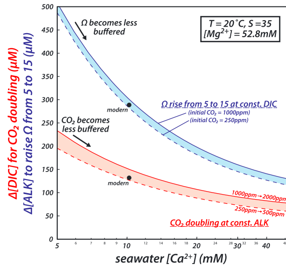
Figure 6. DIC and ALK change required to (red) double CO 2 and to (blue) raise Ω from 5 to 15 strongly decrease as seawater [Ca 2+ ] concentration rises. The initial seawater is set to a CO 2 level of (dashed lines) 250 ppm or (solid lines) 1000 ppm, with Ω set to 5 in both cases.
