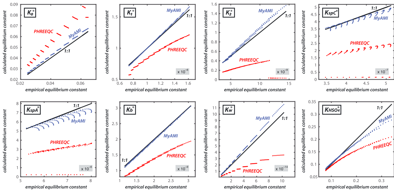
Figure 3. Assessment of model skill by comparison of predicted conditional equilibrium constants of MyAMI (blue; this study) and PHREEQC (red) [Parkhurst, 1995] against the empirical conditional equilibrium constants for modern seawater composition [Weiss, 1974; Lueker et al., 2000; Dickson et al., 1990a, 1990b; Mucci, 1983] in the range of 0–30°C and salinity of 30–40. Our MyAMI model closely tracks the “1:1” line target of perfect agreement with the empirical data. MIAMI model output (not shown) is very similar to MyAMI (see Figure S1). The equilibrium constants documented in this study are made to fully conform to empirical data by using MyAMI only to calculate the change of the equilibrium constants relative to modern seawater (according to supporting information equation (S2)).
