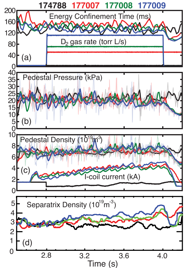
Figure 8. Time evolution of 4 DIII-D shots with varying D_2 gas rates and I-coil feedback control of pedestal density. (a) Energy confinement time (top fluctuating traces) and deuterium gas rate (lower flat traces), (b) pedestal pressure in kPa, (c) pedestal electron density (above) and n = 3 current from the I-coil (below), (d) electron density at the separatrix.
